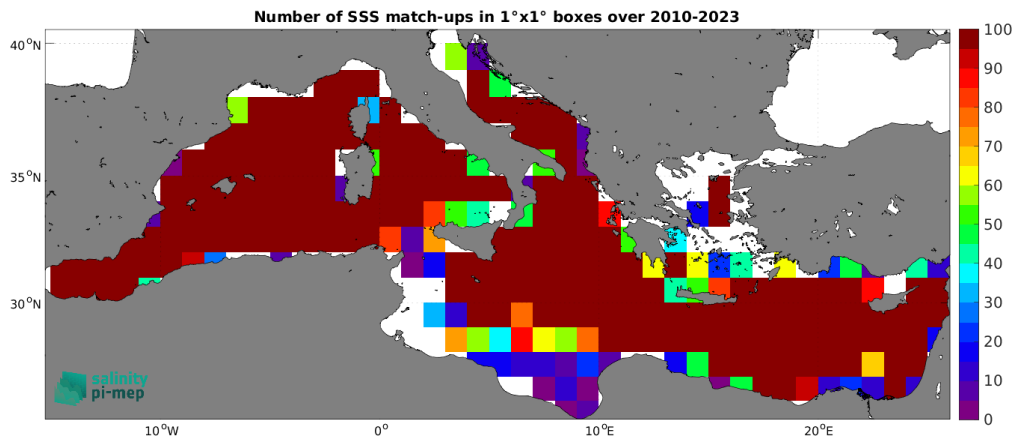
Figure 4: Number of SSS match-ups between Argo SSS and the SMOS SSS L3 v9 - 18 Days (CATDS-CEC-LOCEAN) SSS product for the Mediterranean Sea Pi-MEP region over 1^\circ \times 1^\circ boxes and for the full satellite product period.
