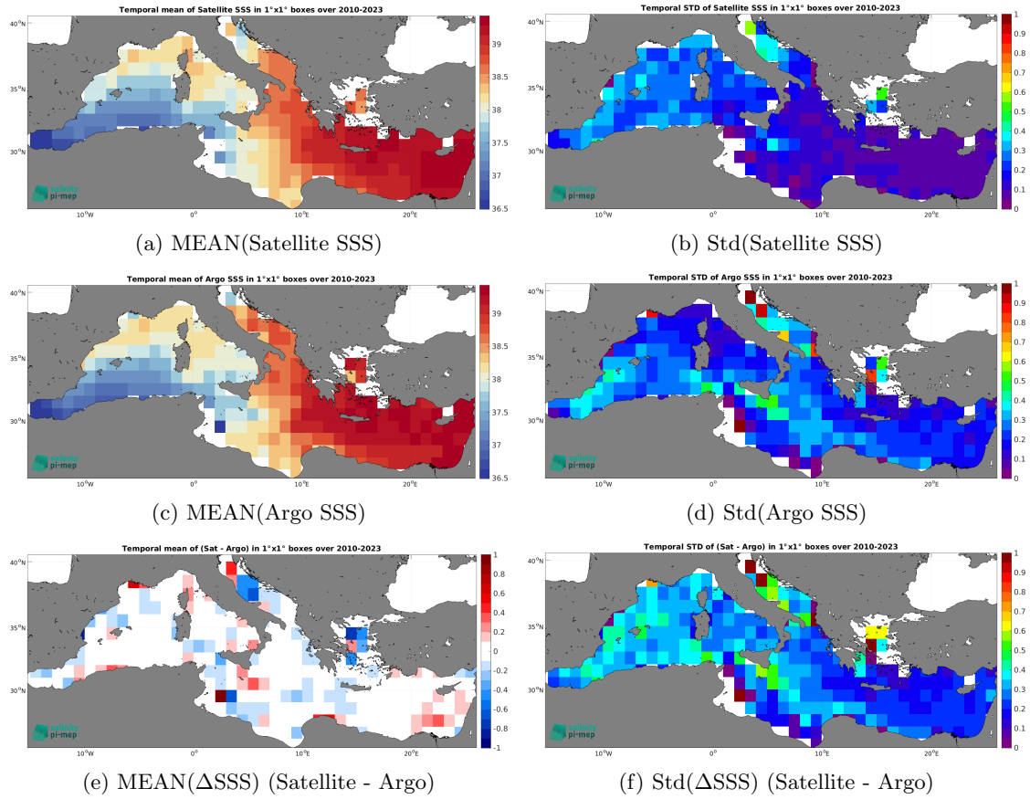
Figure 6: Temporal mean (left) and Std (right) of SSS from SMOS SSS L3 v9 - 18 Days (CATDS-CEC-LOCEAN) (top), Argo (middle), and of \Delta SSS (Satellite - Argo). Only match-up pairs are used to generate these maps.
