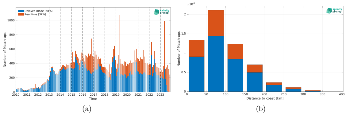
Figure 1: Number of match-ups between Argo and SMOS SSS L3 v9 - 18 Days (CATDS-CEC-LOCEAN) SSS as a function of time (a) and as function of the distance to coast (b) over the Mediterranean Sea Pi-MEP region and for the full satellite product period.
