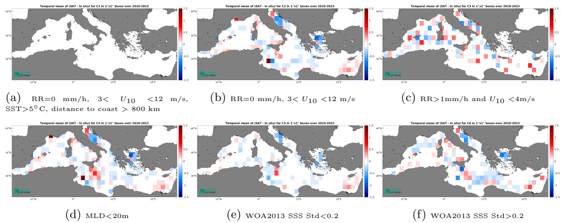
Figure 12: Temporal mean gridded over spatial boxes of size 1^\circ \times 1^\circ of \Delta SSS (SMOS SSS L3 v9 - 18 Days (CATDS-CEC-LOCEAN) - Argo) for 6 different subdatasets corresponding to:RR=0 mm/h, 3 < U_{10} < 12 m/s, SST >5^\circ C, distance to coast > 800 km (a), RR=0 mm/h, 3 < U_{10} < 12 m/s (b), RR >1 mm/h and U_{10} < 4 m/s (c),MLD <20 m (d),WOA2013 SSS Std <0.2 (e),WOA2013 SSS Std >0.2 (f).
