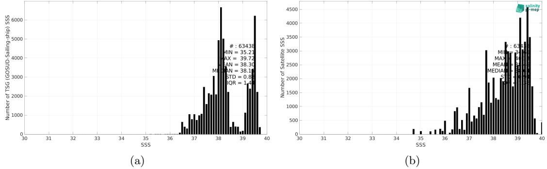
Figure 2: Histograms of SSS from TSG (GOSUD-Sailing-ship) (a) and SMOS SSS L3 v8 - 9 Days (CATDS-CEC-LOCEAN) (b) considering all match-up pairs per bins of 0.1 over the Mediterranean Sea Pi-MEP region and for the full satellite product period.
