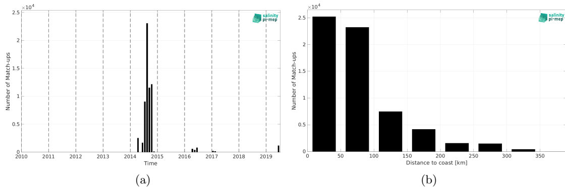
Figure 1: Number of match-ups between TSG (GOSUD-Sailing-ship) and SMOS SSS L3 v8 - 9 Days (CATDS-CEC-LOCEAN) SSS as a function of time (a) and as function of the distance to coast (b) over the Mediterranean Sea Pi-MEP region and for the full satellite product period.
