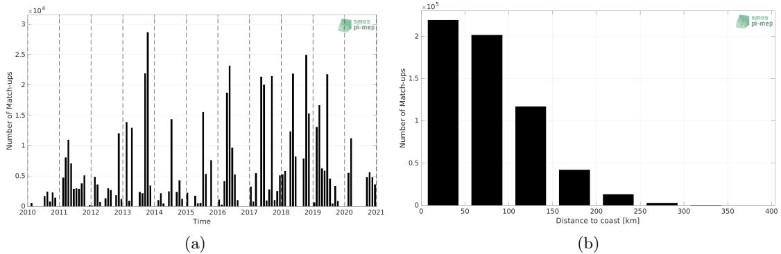
Figure 1: Number of match-ups between TSG (GOSUD-Research-vessel) and SMOS SSS L3 v8 - 9 Days (CATDS-CECOS-LOCEAN) SSS as a function of time (a) and as function of the distance to coast (b) over the Mediterranean Sea Pi-MEP region and for the full satellite product period.
