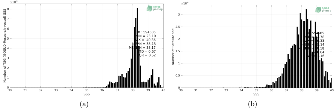
Figure 2: Histograms of SSS from TSG (GOSUD-Research-vessel) (a) and SMOS SSS L3 v8 - 9 Days (CATDS-CECOS-LOCEAN) (b) considering all match-up pairs per bins of 0.1 over the Mediterranean Sea Pi-MEP region and for the full satellite product period.
