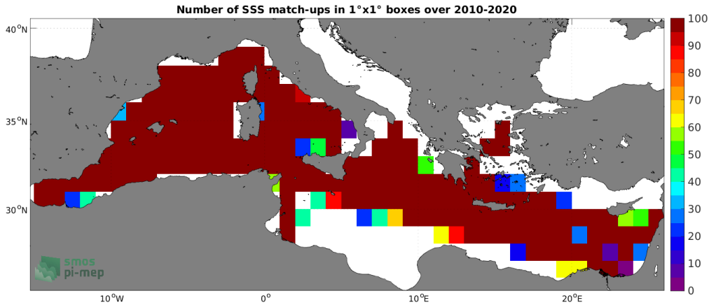
Figure 4: Number of SSS match-ups between TSG (GOSUD-Research-vessel) SSS and the SMOS SSS L3 v8 - 9 Days (CATDS-CECOS-LOCEAN) SSS product for the Mediterranean Sea Pi-MEP region over 1^\circ \times 1^\circ boxes and for the full satellite product period.
