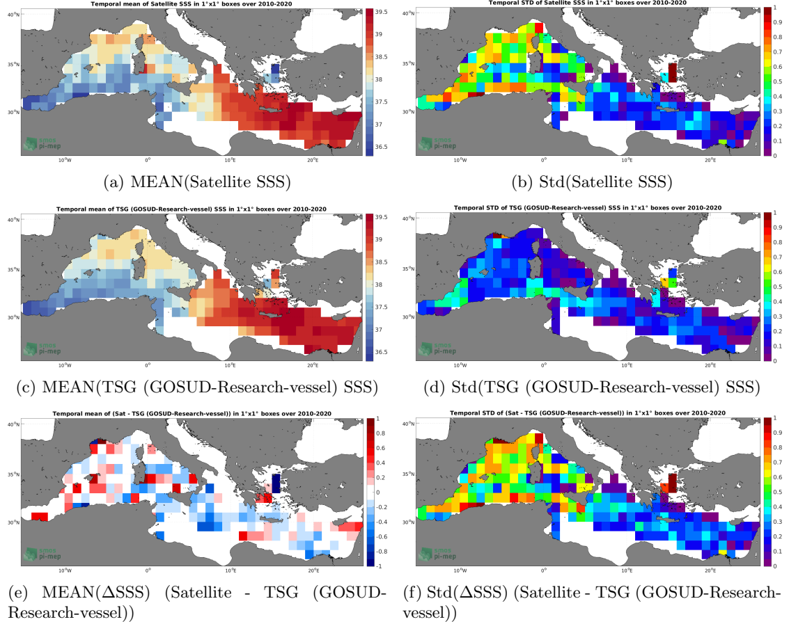
Figure 6: Temporal mean (left) and Std (right) of SSS from SMOS SSS L3 v8 - 9 Days (CATDS-CECOS-LOCEAN) (top), TSG (GOSUD-Research-vessel) (middle), and of \Delta\text{SSS} (Satellite - TSG (GOSUD-Research-vessel)). Only match-up pairs are used to generate these maps.
