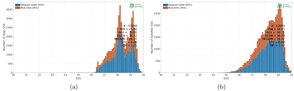
Figure 2: Histograms of SSS from Argo (a) and SMOS SSS L3 v8 - 9 Days (CATDS-CECOS-LOCEAN) (b) considering all match-up pairs per bins of 0.1 over the Mediterranean Sea Pi-MEP region and for the full satellite product period.
