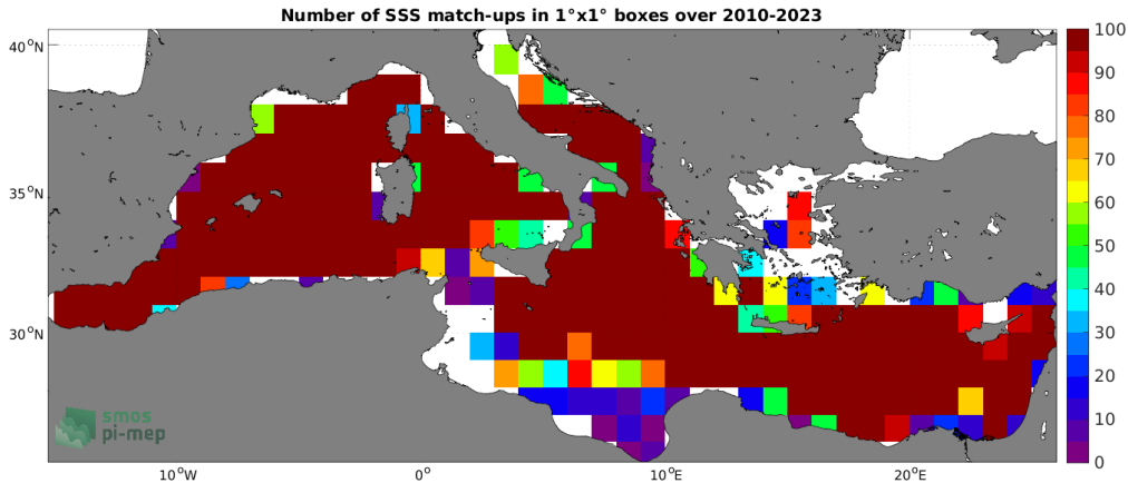
Figure 4: Number of SSS match-ups between Argo SSS and the SMOS SSS L3 v8 - 9 Days (CATDS-CECOS-LOCEAN) SSS product for the Mediterranean Sea Pi-MEP region over 1^\circ \times 1^\circ boxes and for the full satellite product period.
