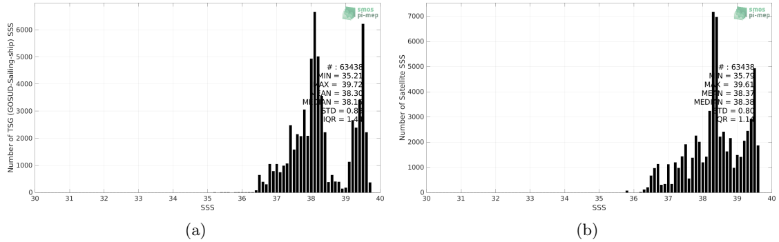
Figure 2: Histograms of SSS from TSG (GOSUD-Sailing-ship) (a) and SMOS SSS L3 v8 - 18 Days (CATDS-CECOS-LOCEAN) (b) considering all match-up pairs per bins of 0.1 over the Mediterranean Sea Pi-MEP region and for the full satellite product period.
