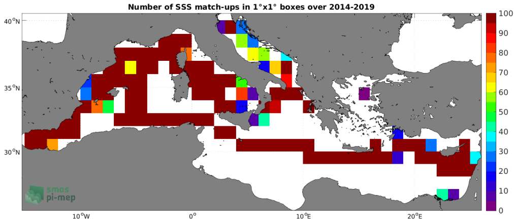
Figure 4: Number of SSS match-ups between TSG (GOSUD-Sailing-ship) SSS and the SMOS SSS L3 v8 - 18 Days (CATDS-CECOS-LOCEAN) SSS product for the Mediterranean Sea Pi-MEP region over 1^\circ \times 1^\circ boxes and for the full satellite product period.
