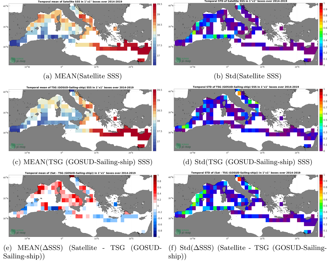
Figure 6: Temporal mean (left) and Std (right) of SSS from SMOS SSS L3 v8 - 18 Days (CATDS-CECOS-LOCEAN) (top), TSG (GOSUD-Sailing-ship) (middle), and of \Delta\text{SSS} (Satellite - TSG (GOSUD-Sailing-ship)). Only match-up pairs are used to generate these maps.
