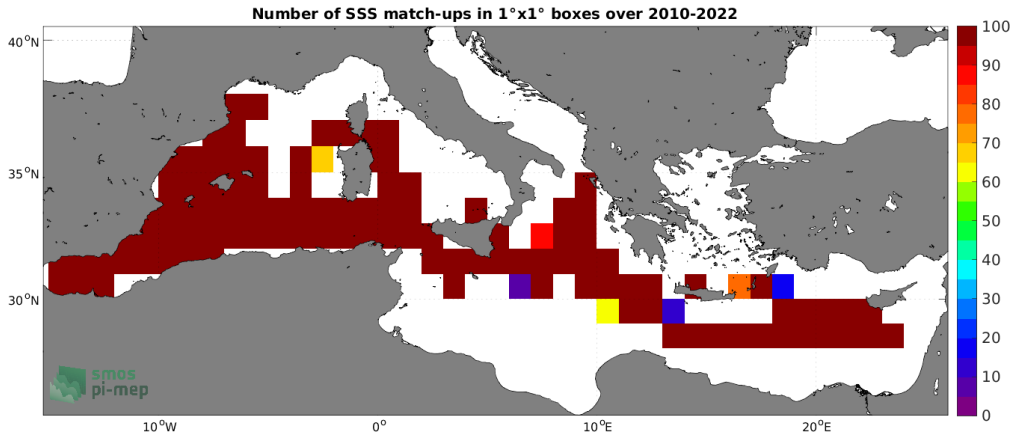
Figure 4: Number of SSS match-ups between TSG (CSIC-UTM) SSS and the SMOS SSS L3 v8 - 18 Days (CATDS-CECOS-LOCEAN) SSS product for the Mediterranean Sea Pi-MEP region over 1^\circ \times 1^\circ boxes and for the full satellite product period.
