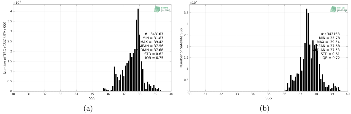
Figure 2: Histograms of SSS from TSG (CSIC-UTM) (a) and SMOS SSS L3 v8 - 18 Days (CATDS-CECOS-LOCEAN) (b) considering all match-up pairs per bins of 0.1 over the Mediterranean Sea Pi-MEP region and for the full satellite product period.
