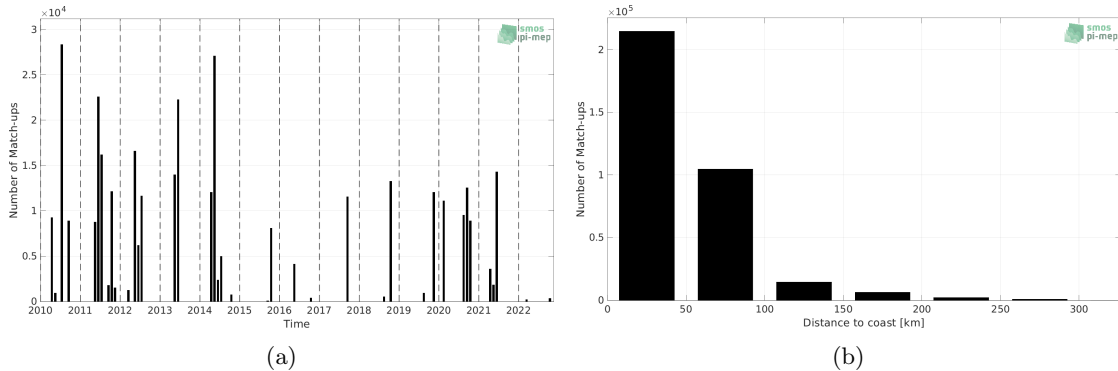
Figure 1: Number of match-ups between TSG (CSIC-UTM) and SMOS SSS L3 v8 - 18 Days (CATDS-CECOS-LOCEAN) SSS as a function of time (a) and as function of the distance to coast (b) over the Mediterranean Sea Pi-MEP region and for the full satellite product period.
