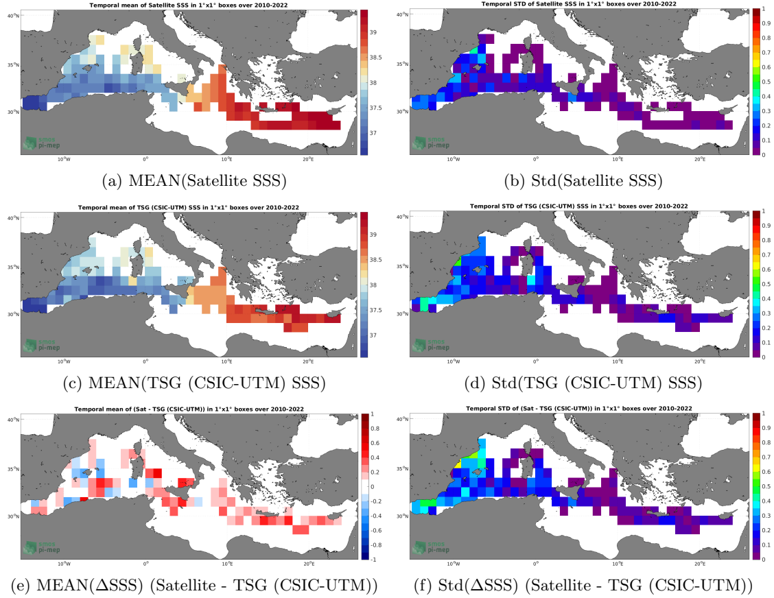
Figure 6: Temporal mean (left) and Std (right) of SSS from SMOS SSS L3 v8 - 18 Days (CATDS-CECOS-LOCEAN) (top), TSG (CSIC-UTM) (middle), and of \Delta\text{SSS} (Satellite - TSG (CSIC-UTM)). Only match-up pairs are used to generate these maps.
