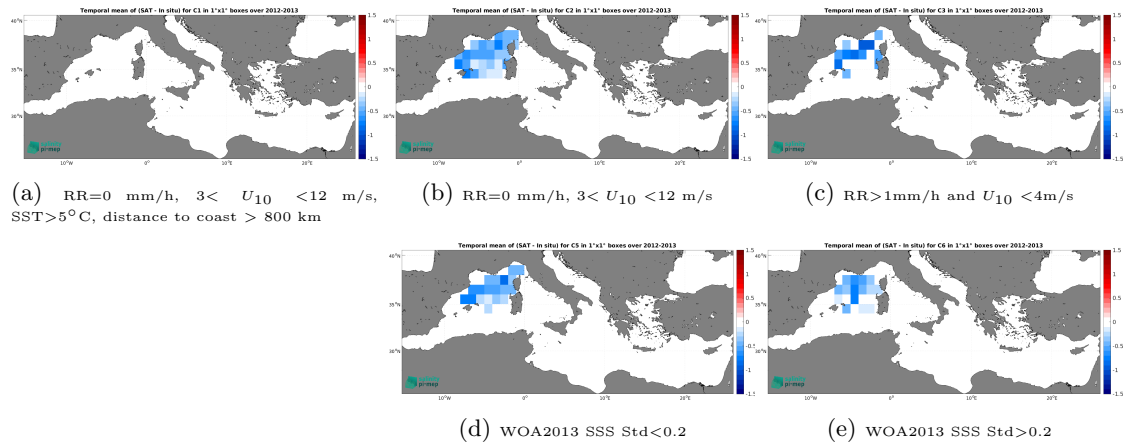
Figure 11: Temporal mean gridded over spatial boxes of size 1^{\circ}\times 1^{\circ} of \Delta\text{SSS} (SMOS SSS L3 v8 - 18 Days (CATDS-CEC-LOCEAN) - Surface drifters) for 5 different subdatasets corresponding to: RR=0 mm/h, 3 < U_{10} < 12 m/s, SST > 5^{\circ}\text{C} , distance to coast > 800 km (a), RR=0 mm/h, 3 < U_{10} < 12 m/s (b), RR > 1 mm/h and U_{10} < 4 m/s (c), WOA2013 SSS Std < 0.2 (d), WOA2013 SSS Std > 0.2 (e).
