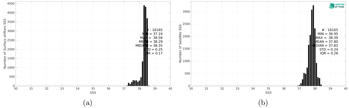
Figure 2: Histograms of SSS from Surface drifters (a) and SMOS SSS L3 v8 - 18 Days (CATDS-CEC-LOCEAN) (b) considering all match-up pairs per bins of 0.1 over the Mediterranean Sea Pi-MEP region and for the full satellite product period.
