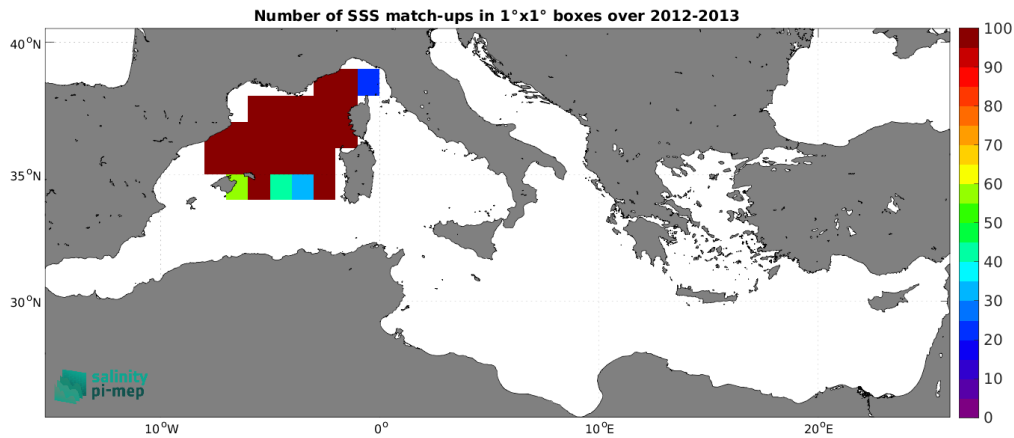
Figure 3: Number of SSS match-ups between Surface drifters SSS and the SMOS SSS L3 v8 - 18 Days (CATDS-CEC-LOCEAN) SSS product for the Mediterranean Sea Pi-MEP region over 1^\circ \times 1^\circ boxes and for the full satellite product period.
