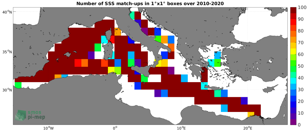
Figure 4: Number of SSS match-ups between TSG (LEGOS-DM) SSS and the SMOS SSS L3 v7 - 9 Days (CATDS-CECOS-LOCEAN) SSS product for the Mediterranean Sea Pi-MEP region over 1^\circ \times 1^\circ boxes and for the full satellite product period.
