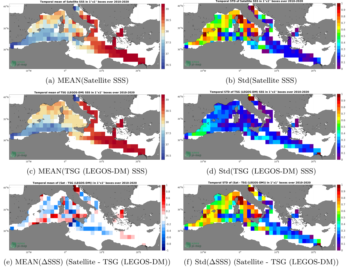
Figure 6: Temporal mean (left) and Std (right) of SSS from SMOS SSS L3 v7 - 9 Days (CATDS-CECOS-LOCEAN) (top), TSG (LEGOS-DM) ( in situ ) dataset (middle), and of \Delta\text{SSS} (Satellite - TSG (LEGOS-DM)). Only match-up pairs are used to generate these maps.
