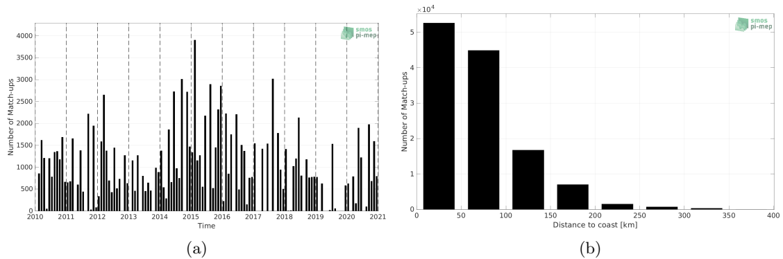
Figure 1: Number of match-ups between TSG (LEGOS-DM) and SMOS SSS L3 v7 - 9 Days (CATDS-CECOS-LOCEAN) SSS as a function of time (a) and as function of the distance to coast (b) over the Mediterranean Sea Pi-MEP region and for the full satellite product period.
