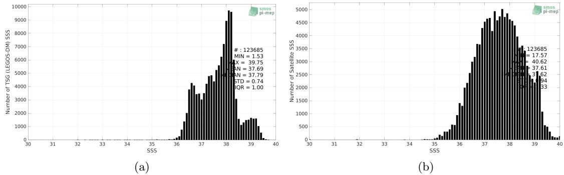
Figure 2: Histograms of SSS from TSG (LEGOS-DM) (a) and SMOS SSS L3 v7 - 9 Days (CATDS-CECOS-LOCEAN) (b) considering all match-up pairs per bins of 0.1 over the Mediterranean Sea Pi-MEP region and for the full satellite product period.
