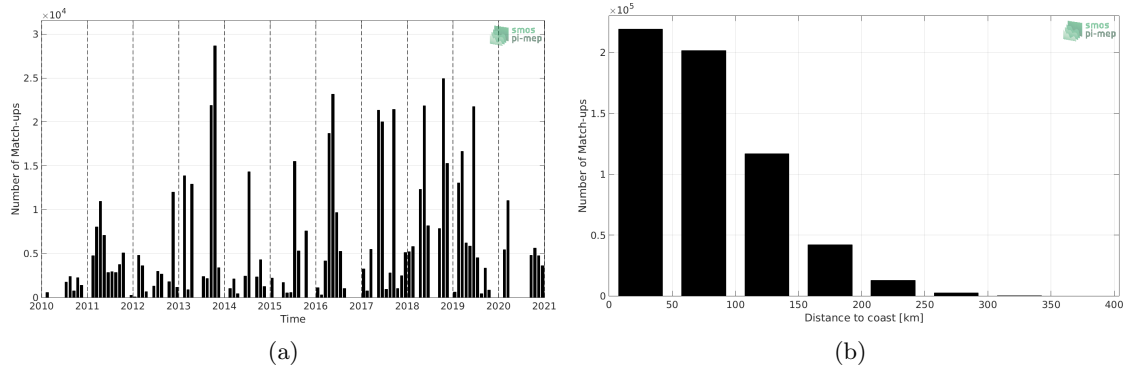
Figure 1: Number of match-ups between TSG (GOSUD-Research-vessel) and SMOS SSS L3 v7 - 9 Days (CATDS-CECOS-LOCEAN) SSS as a function of time (a) and as function of the distance to coast (b) over the Mediterranean Sea Pi-MEP region and for the full satellite product period.
