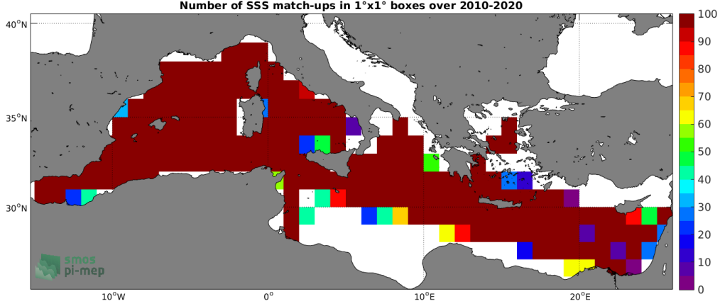
Figure 4: Number of SSS match-ups between TSG (GOSUD-Research-vessel) SSS and the SMOS SSS L3 v7 - 9 Days (CATDS-CECOS-LOCEAN) SSS product for the Mediterranean Sea Pi-MEP region over 1^\circ \times 1^\circ boxes and for the full satellite product period.
