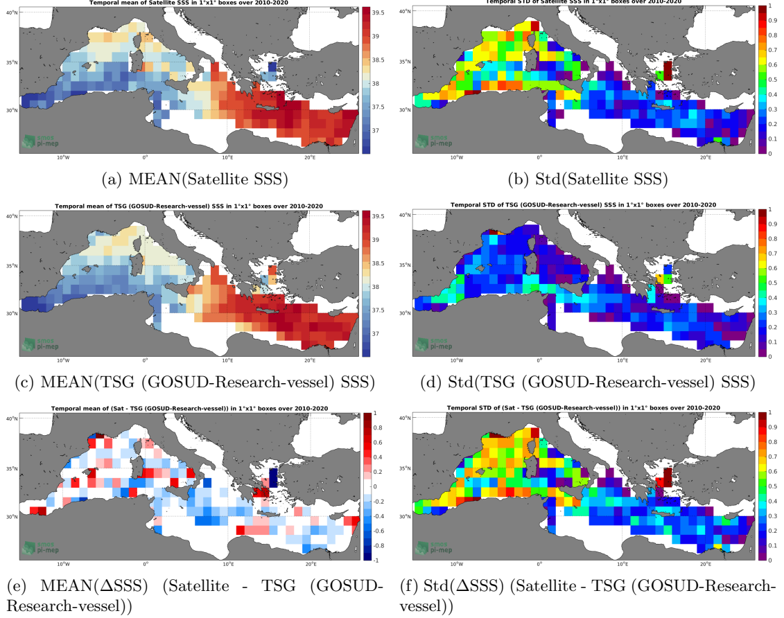
Figure 6: Temporal mean (left) and Std (right) of SSS from SMOS SSS L3 v7 - 9 Days (CATDS-CECOS-LOCEAN) (top), TSG (GOSUD-Research-vessel) (middle), and of \Delta\text{SSS} (Satellite - TSG (GOSUD-Research-vessel)). Only match-up pairs are used to generate these maps.
