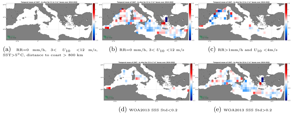
Figure 12: Temporal mean gridded over spatial boxes of size 1^\circ \times 1^\circ of \Delta SSS (SMOS SSS L3 v7 - 9 Days (CATDS-CECOS-LOCEAN) - TSG (GOSUD-Research-vessel)) for 5 different subdatasets corresponding to: RR=0 mm/h, 3 < U_{10} < 12 m/s, SST > 5^\circ\text{C} , distance to coast > 800 km (a), RR=0 mm/h, 3 < U_{10} < 12 m/s (b), RR > 1 mm/h and U_{10} < 4 m/s (c), WOA2013 SSS Std < 0.2 (d), WOA2013 SSS Std > 0.2 (e).
