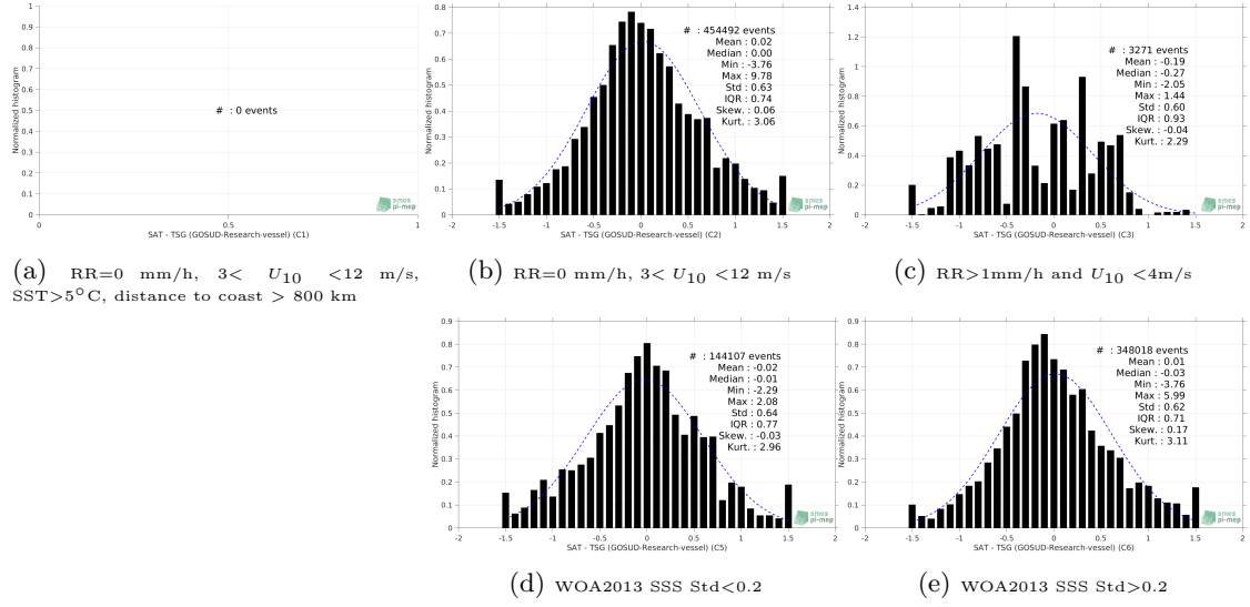
Figure 13: Normalized histogram of \Delta\text{SSS} (SMOS SSS L3 v7 - 9 Days (CATDS-CECOS-LOCEAN) - TSG (GOSUD-Research-vessel)) for 5 different subdatasets corresponding to: RR=0 mm/h, 3 < U_{10} < 12 m/s, SST > 5^\circ\text{C} , distance to coast > 800 km (a), RR=0 mm/h, 3 < U_{10} < 12 m/s (b), RR > 1\text{mm/h} and U_{10} < 4\text{m/s} (c), WOA2013 SSS Std <0.2 (d), WOA2013 SSS Std >0.2 (e).
