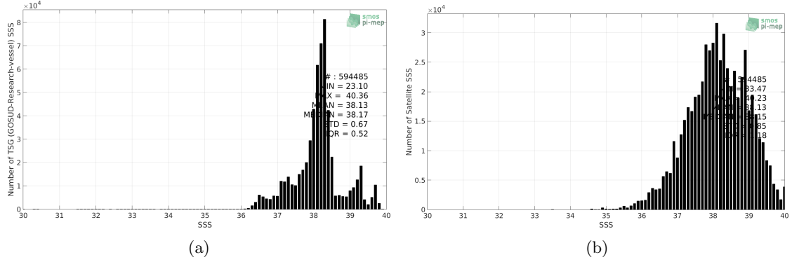
Figure 2: Histograms of SSS from TSG (GOSUD-Research-vessel) (a) and SMOS SSS L3 v7 - 9 Days (CATDS-CECOS-LOCEAN) (b) considering all match-up pairs per bins of 0.1 over the Mediterranean Sea Pi-MEP region and for the full satellite product period.
