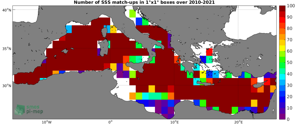
Figure 4: Number of SSS match-ups between Argo SSS and the SMOS SSS L3 v7 - 9 Days (CATDS-CECOS-LOCEAN) SSS product for the Mediterranean Sea Pi-MEP region over 1^\circ \times 1^\circ boxes and for the full satellite product period.
