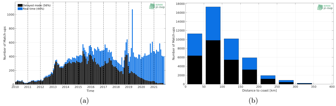
Figure 1: Number of match-ups between Argo and SMOS SSS L3 v7 - 9 Days (CATDS-CECOS-LOCEAN) SSS as a function of time (a) and as function of the distance to coast (b) over the Mediterranean Sea Pi-MEP region and for the full satellite product period.
