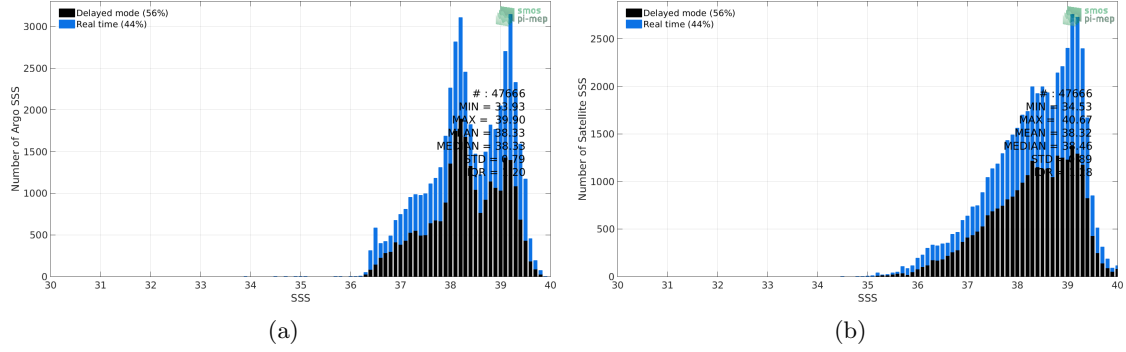
Figure 2: Histograms of SSS from Argo (a) and SMOS SSS L3 v7 - 9 Days (CATDS-CECOS-LOCEAN) (b) considering all match-up pairs per bins of 0.1 over the Mediterranean Sea Pi-MEP region and for the full satellite product period.
