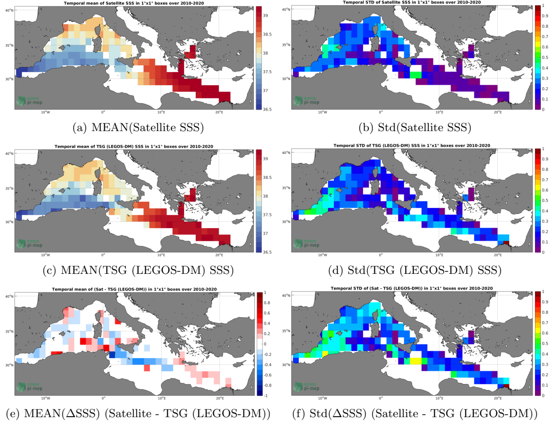
Figure 6: Temporal mean (left) and Std (right) of SSS from SMOS SSS L3 v7 - 18 Days (CATDS-CECOS-LOCEAN) (top), TSG (LEGOS-DM) (middle), and of \Delta\text{SSS} (Satellite - TSG (LEGOS-DM)). Only match-up pairs are used to generate these maps.
