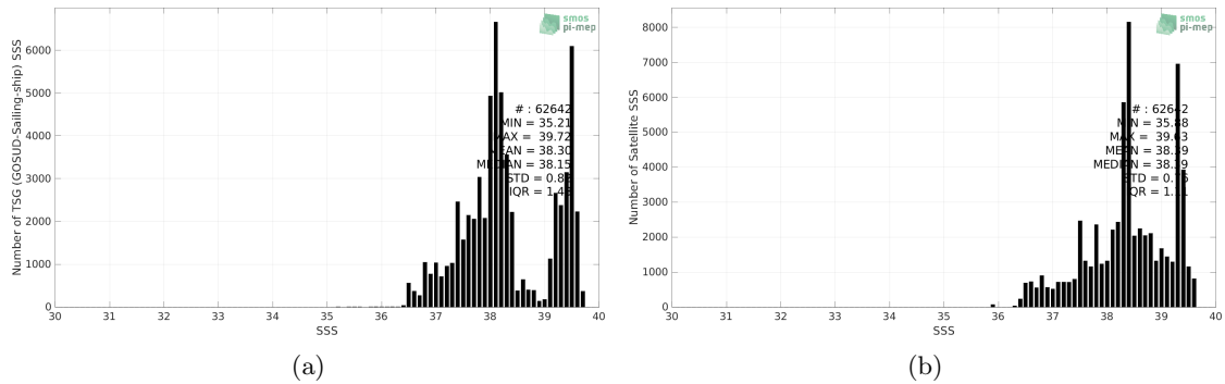
Figure 2: Histograms of SSS from TSG (GOSUD-Sailing-ship) (a) and SMOS SSS L3 v7 - 18 Days (CATDS-CECOS-LOCEAN) (b) considering all match pairs per bins of 0.1 over the Mediterranean Sea Pi-MEP region and for the full satellite product period.
