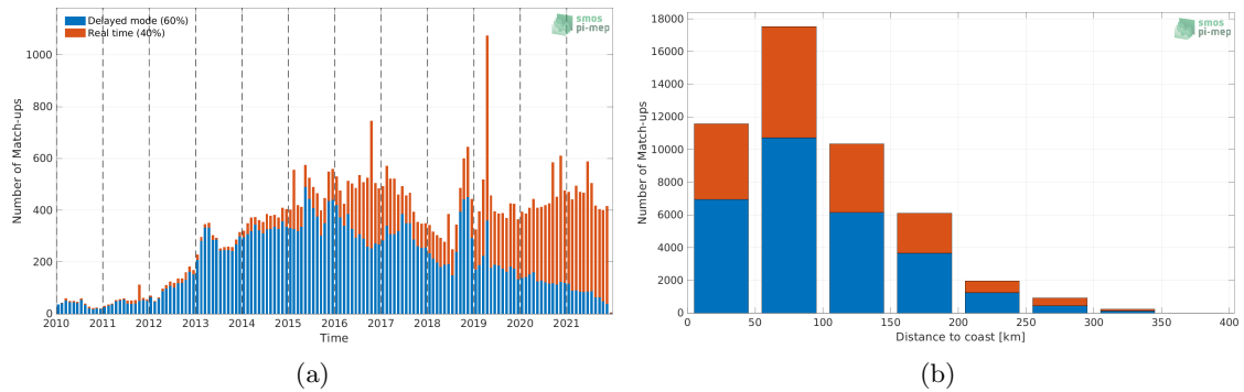
Figure 1: Number of match-ups between Argo and SMOS SSS L3 v7 - 18 Days (CATDS-CECOS-LOCEAN) SSS as a function of time (a) and as function of the distance to coast (b) over the Mediterranean Sea Pi-MEP region and for the full satellite product period.
