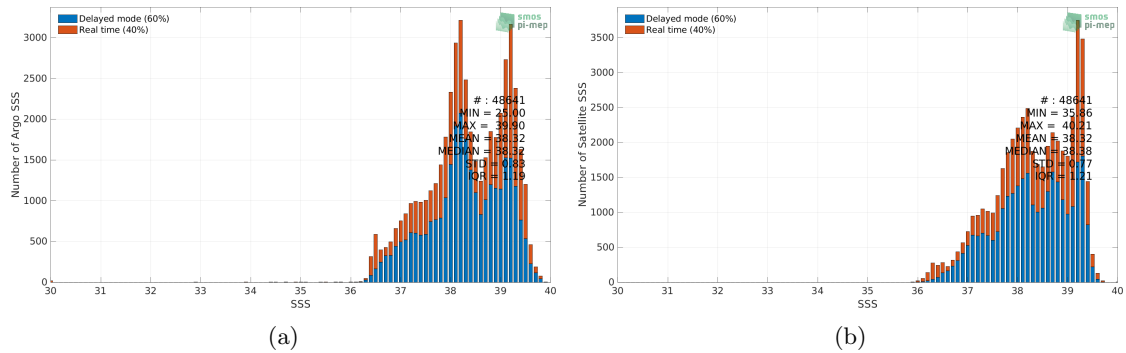
Figure 2: Histograms of SSS from Argo (a) and SMOS SSS L3 v7 - 18 Days (CATDS-CECOS-LOCEAN) (b) considering all match-up pairs per bins of 0.1 over the Mediterranean Sea Pi-MEP region and for the full satellite product period.
