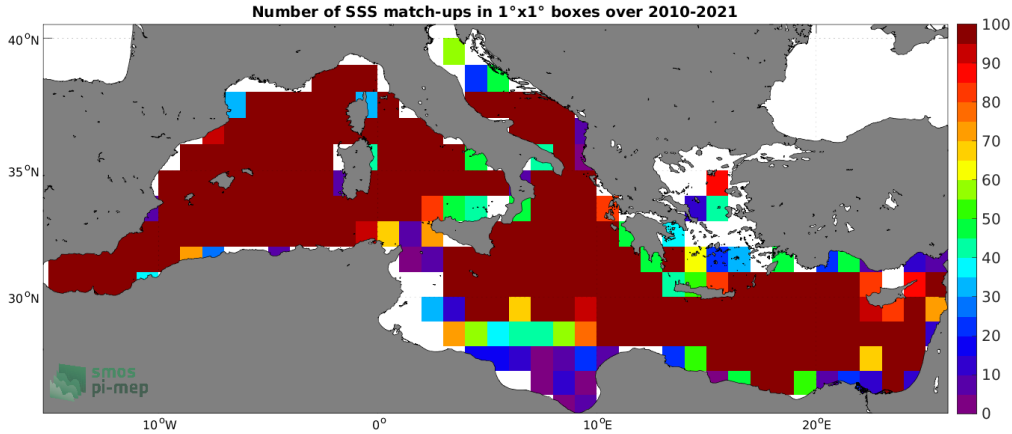
Figure 4: Number of SSS match-ups between Argo SSS and the SMOS SSS L3 v7 - 18 Days (CATDS-CECOS-LOCEAN) SSS product for the Mediterranean Sea Pi-MEP region over 1^\circ \times 1^\circ boxes and for the full satellite product period.
