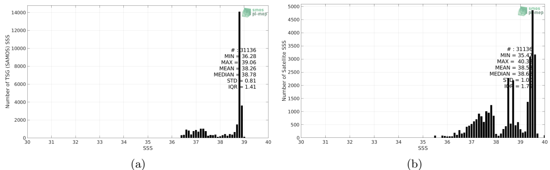
Figure 2: Histograms of SSS from TSG (SAMOS) (a) and SMOS SSS L3 v5 - 9 Days (CATDS-CECOS-LOCEAN) (b) considering all match-up pairs per bins of 0.1 over the Mediterranean Sea Pi-MEP region and for the full satellite product period.
