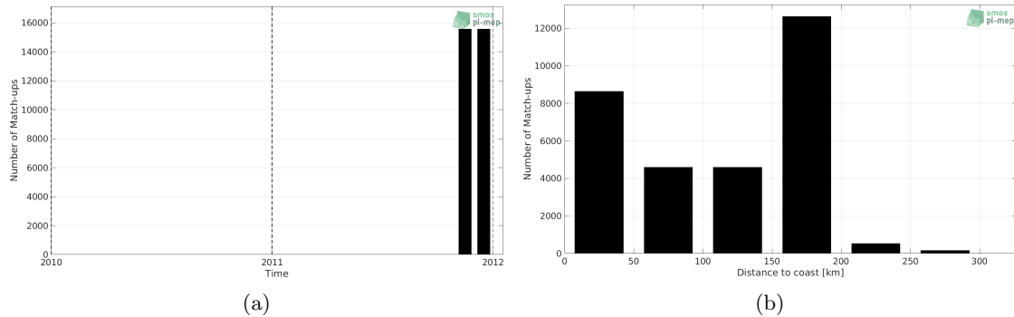
Figure 1: Number of match-ups between TSG (SAMOS) and SMOS SSS L3 v5 - 9 Days (CATDS-CECOS-LOCEAN) SSS as a function of time (a) and as function of the distance to coast (b) over the Mediterranean Sea Pi-MEP region and for the full satellite product period.
