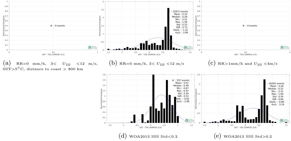
Figure 13: Normalized histogram of \Delta SSS (SMOS SSS L3 v5 - 9 Days (CATDS-CECOS-LOCEAN) - TSG (SAMOS)) for 5 different subdatasets corresponding to: RR=0 mm/h, 3 < U_{10} < 12 m/s, SST > 5°C, distance to coast > 800 km (a), RR=0 mm/h, 3 < U_{10} < 12 m/s (b), RR > 1mm/h and U_{10} < 4 m/s (c), WOA2013 SSS Std < 0.2 (d), WOA2013 SSS Std > 0.2 (e).
