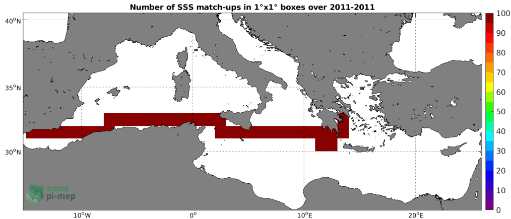
Figure 4: Number of SSS match-ups between TSG (SAMOS) SSS and the SMOS SSS L3 v5 - 9 Days (CATDS-CECOS-LOCEAN) SSS product for the Mediterranean Sea Pi-MEP region over 1^\circ \times 1^\circ boxes and for the full satellite product period.
