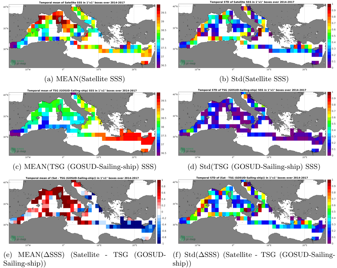
Figure 6: Temporal mean (left) and Std (right) of SSS from SMOS SSS L3 v5 - 9 Days (CATDS-CECOS-LOCEAN) (top), TSG (GOSUD-Sailing-ship) (middle), and of \Delta\text{SSS} (Satellite - TSG (GOSUD-Sailing-ship)). Only match-up pairs are used to generate these maps.
