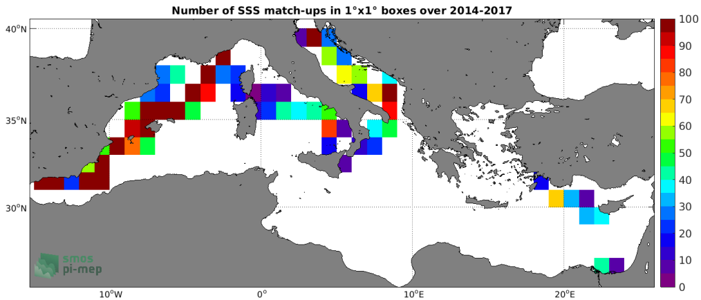
Figure 4: Number of SSS match-ups between TSG (GOSUD-Sailing-ship) SSS and the SMOS SSS L3 v5 - 9 Days (CATDS-CECOS-LOCEAN) SSS product for the Mediterranean Sea Pi-MEP region over 1°x1° boxes and for the full satellite product period.
