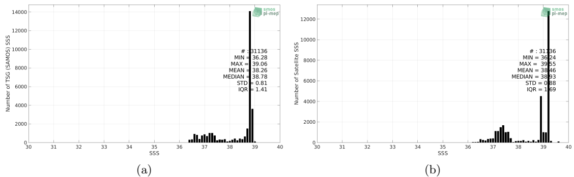
Figure 2: Histograms of SSS from TSG (SAMOS) (a) and SMOS SSS L3 v5 - 18 Days (CATDS-CECOS-LOCEAN) (b) considering all match-up pairs per bins of 0.1 over the Mediterranean Sea Pi-MEP region and for the full satellite product period.
