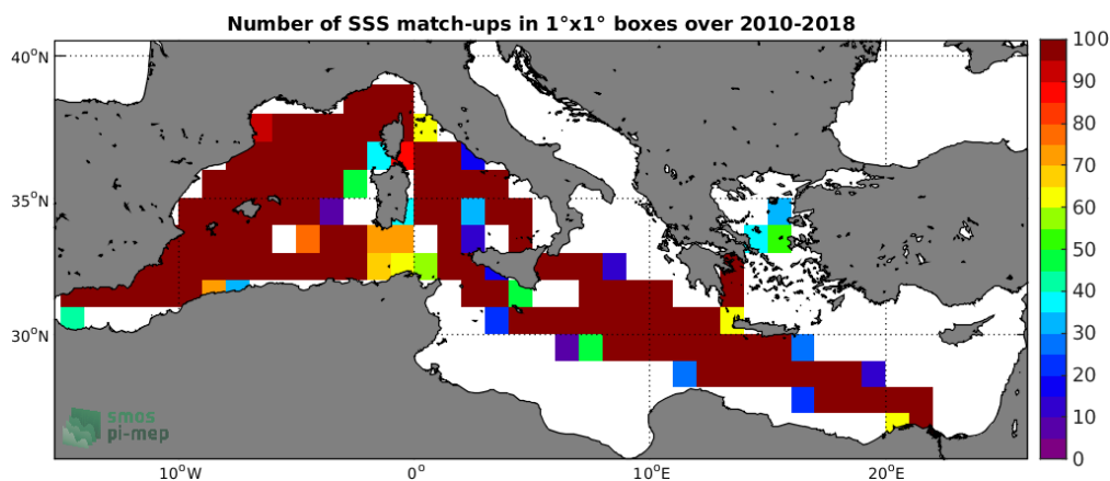
Figure 4: Number of SSS match-ups between TSG-LEGOS-DM SSS and the SMOS-L3-CATDS-CECOS-LOCEAN-V4-9DAYS-25KM SSS product for the Mediterranean Sea Pi-MEP region over 1°x1° boxes and for the full satellite product period.
