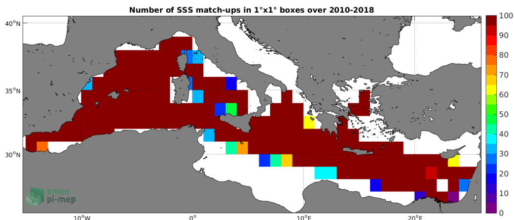
Figure 4: Number of SSS match-ups between TSG-GOSUD-Research-vessel SSS and the SMOS-L3-CATDS-CECOS-LOCEAN-V4-9DAYS-25KM SSS product for the Mediterranean Sea Pi-MEP region over 1^\circ \times 1^\circ boxes and for the full satellite product period.
