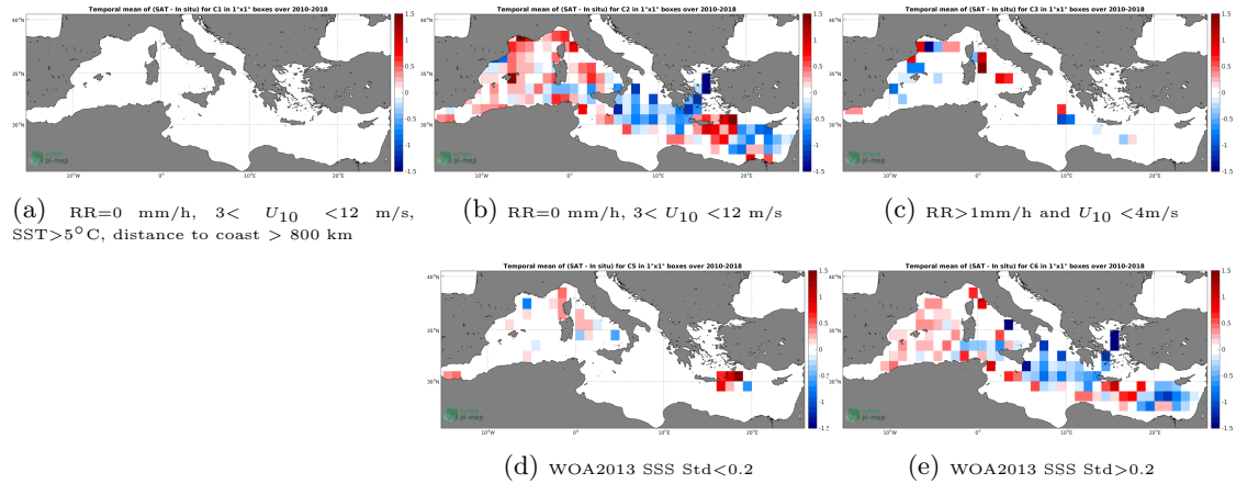
Figure 12: Temporal mean gridded over spatial boxes of size 1^{\circ}\times 1^{\circ} of \Delta SSS (SMOS-L3-CATDS-CECOS-LOCEAN-V4-9DAYS-25KM - TSG-GOSUD-Research-vessel) for 5 different subdatasets corresponding to:RR=0 mm/h, 3 < U_{10} < 12 m/s, SST >5^{\circ}\text{C} , distance to coast > 800 km (a), RR=0 mm/h, 3 < U_{10} < 12 m/s (b), RR >1 mm/h and U_{10} < 4 m/s (c), WOA2013 SSS Std <0.2 (d), WOA2013 SSS Std >0.2 (e).
