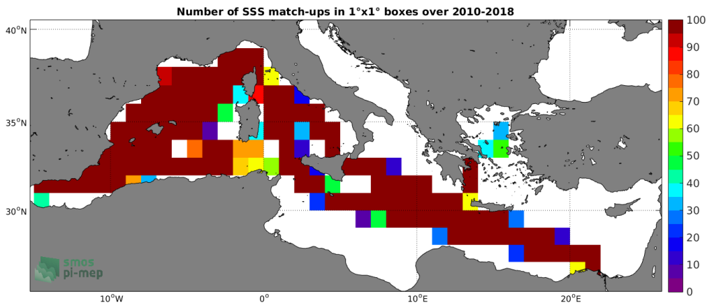
Figure 4: Number of SSS match-ups between TSG (LEGOS-DM) SSS and the SMOS SSS L3 v4 - 18 Days (CATDS-CECOS-LOCEAN) SSS product for the Mediterranean Sea Pi-MEP region over 1°x1° boxes and for the full satellite product period.
