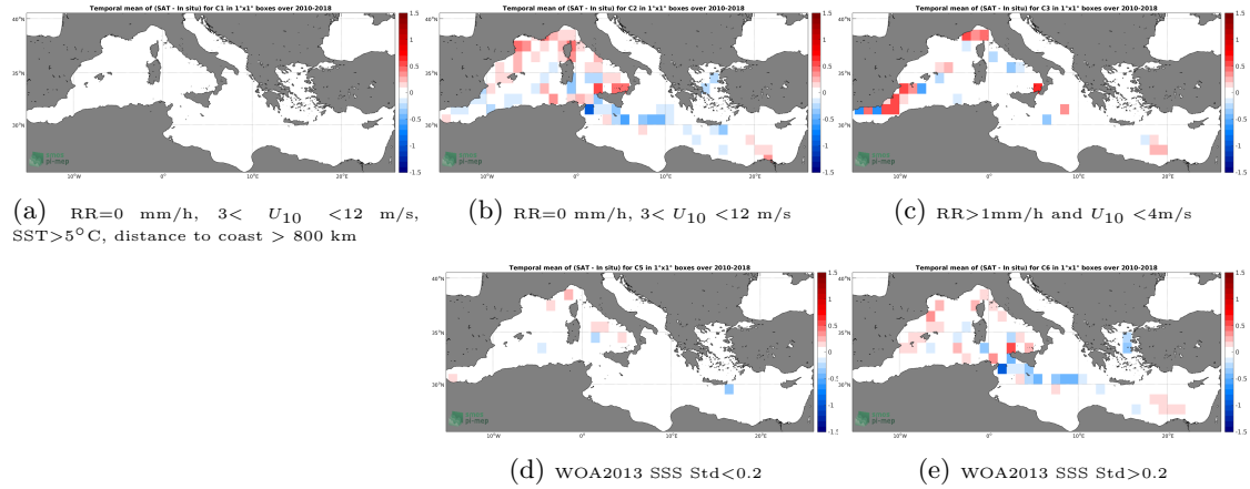
Figure 12: Temporal mean gridded over spatial boxes of size 1^{\circ}\times 1^{\circ} of \Delta\text{SSS} (SMOS SSS L3 v4 - 18 Days (CATDS-CECOS-LOCEAN) - TSG (LEGOS-DM)) for 5 different subdatasets corresponding to:RR=0 mm/h, 3 < U_{10} < 12 m/s, SST >5^{\circ}\text{C} , distance to coast > 800 km (a), RR=0 mm/h, 3 < U_{10} < 12 m/s (b), RR >1 mm/h and U_{10} < 4 m/s (c), WOA2013 SSS Std <0.2 (d), WOA2013 SSS Std >0.2 (e).
