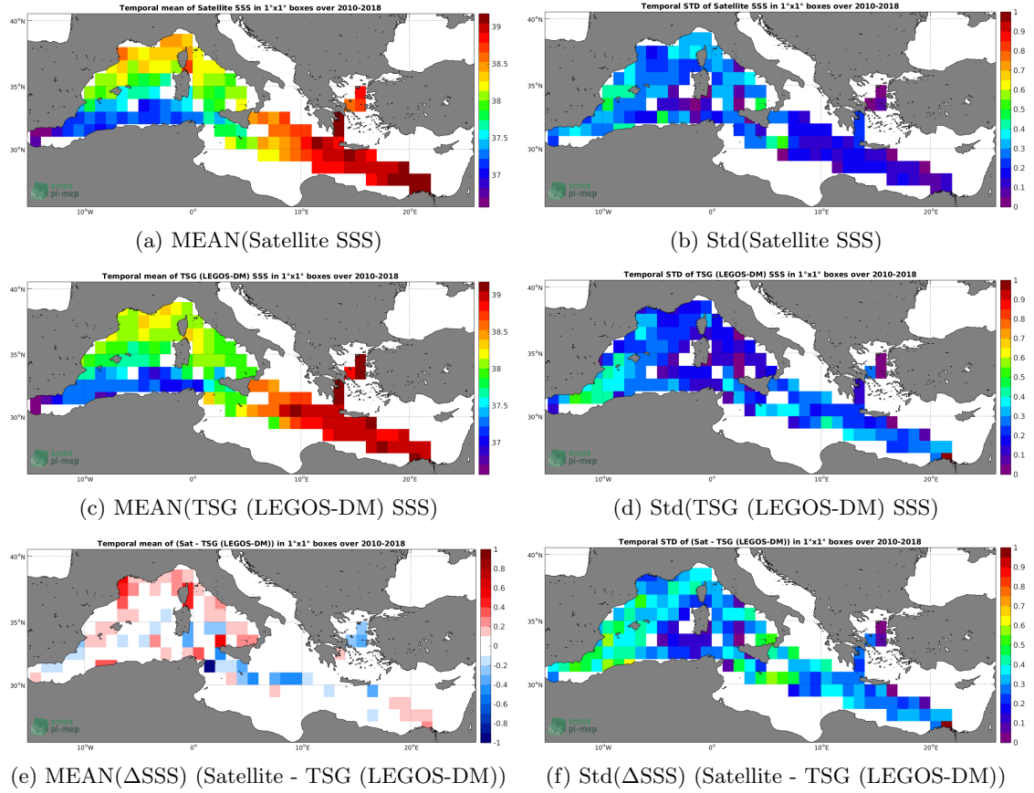
Figure 6: Temporal mean (left) and Std (right) of SSS from SMOS SSS L3 v4 - 18 Days (CATDS-CECOS-LOCEAN) (top), TSG (LEGOS-DM) ( in situ ) dataset (middle), and of \Delta SSS (Satellite - TSG (LEGOS-DM)). Only match-up pairs are used to generate these maps.
