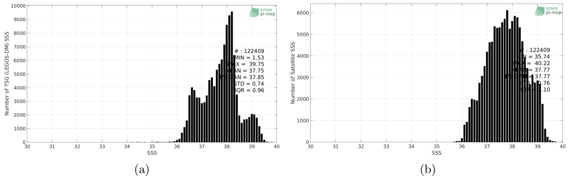
Figure 2: Histograms of SSS from TSG (LEGOS-DM) (a) and SMOS SSS L3 v4 - 18 Days (CATDS-CECOS-LOCEAN) (b) considering all match-up pairs per bins of 0.1 over the Mediterranean Sea Pi-MEP region and for the full satellite product period.
