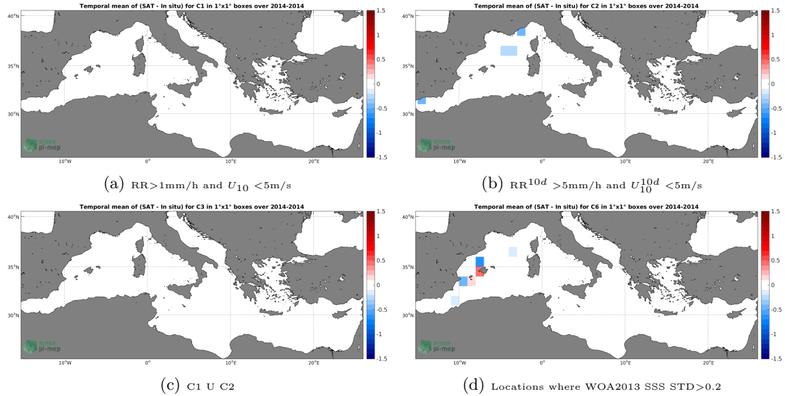
Figure 12: Temporal mean gridded over spatial boxes of size 1^\circ \times 1^\circ of \Delta SSS (SMOS-L3-CATDS-CECOS-LOCEAN-V3-9DAYS-25KM - TSG-GOSUD-Sailing-ship) for 4 different subdatasets corresponding to: RR > 1mm/h and U_{10} < 5\text{m/s} (a), RR^{10d} > 5\text{mm/h} and U_{10}^{10d} < 5\text{m/s} (b), C1 U C2 (c), Locations where WOA2013 SSS STD > 0.2 (d).
