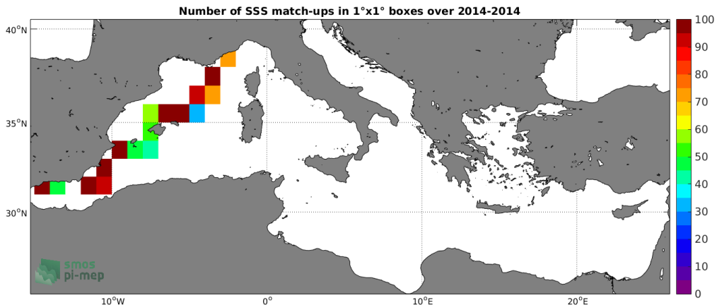
Figure 4: Number of SSS match-ups between TSG-GOSUD-Sailing-ship SSS and the SMOS-L3-CATDS-CECOS-LOCEAN-V3-9DAYS-25KM SSS product for the Mediterranean Sea Pi-MEP region over 1^\circ \times 1^\circ boxes and for the full satellite product period.
