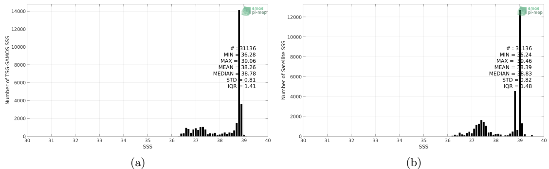
Figure 2: Histograms of SSS from TSG-SAMOS (a) and SMOS-L3-CATDS-CECOS-LOCEAN-V3-18DAYS-25KM (b) considering all match-up pairs per bins of 0.1 over the Mediterranean Sea Pi-MEP region and for the full satellite product period.
