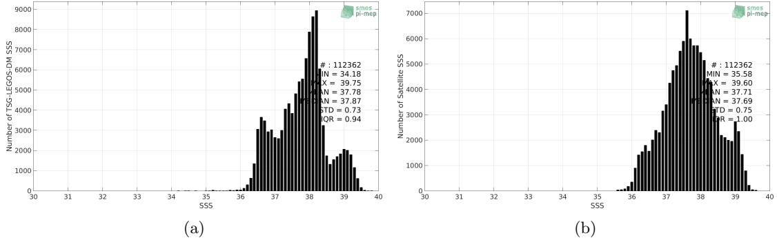
Figure 2: Histograms of SSS from TSG-LEGOS-DM (a) and SMOS-L3-CATDS-CECOS-LOCEAN-V3-18DAYS-25KM (b) considering all match-up pairs per bins of 0.1 over the Mediterranean Sea Pi-MEP region and for the full satellite product period.
