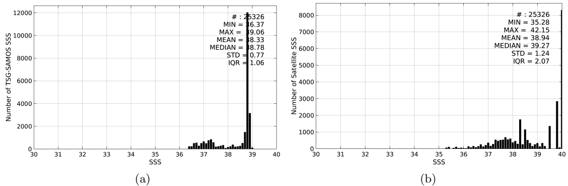
Figure 2: Histograms of SSS from TSG-SAMOS (a) and SMOS-L3-CATDS-CECOS-LOCEAN-V2-9DAYS-25KM (b) considering all match-up pairs per bins of 0.1 over the Mediterranean Sea Pi-MEP region and for the full satellite product period.
