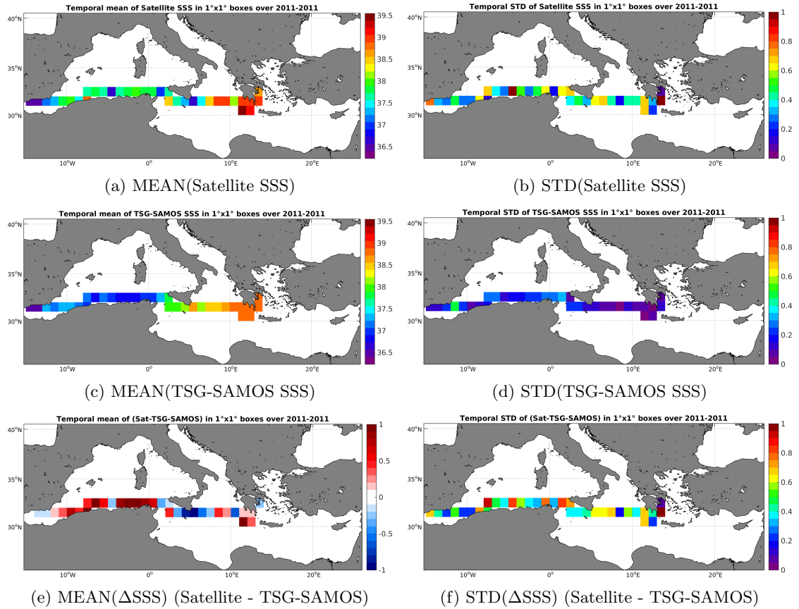
Figure 6: Temporal mean (left) and STD (right) of SSS from SMOS-L3-CATDS-CECOS-LOCEAN-V2-9DAYS-25KM (top), TSG-SAMOS (middle), and of \Delta SSS (Satellite - TSG-SAMOS). Only match-up pairs are used to generate these maps.
