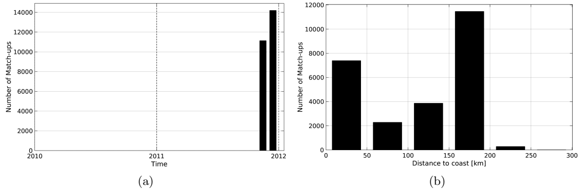
Figure 1: Number of match-ups between TSG-SAMOS and SMOS-L3-CATDS-CECOS-LOCEAN-V2-9DAYS-25KM SSS as a function of time (a) and as function of the distance to coast (b) over the Mediterranean Sea Pi-MEP region and for the full satellite product period.
