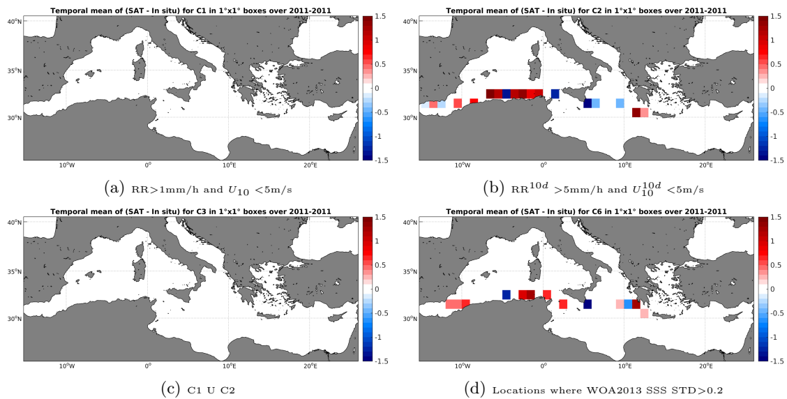
Figure 12: Temporal mean gridded over spatial boxes of size 1^\circ \times 1^\circ of \Delta SSS (SMOS-L3-CATDS-CECOS-LOCEAN-V2-9DAYS-25KM - TSG-SAMOS) for 4 different subdatasets corresponding to: RR > 1\text{mm/h} and U_{10} < 5\text{m/s} (a), RR^{10d} > 5\text{mm/h} and U_{10}^{10d} < 5\text{m/s} (b), C1 U C2 (c), Locations where WOA2013 SSS STD > 0.2 (d).
