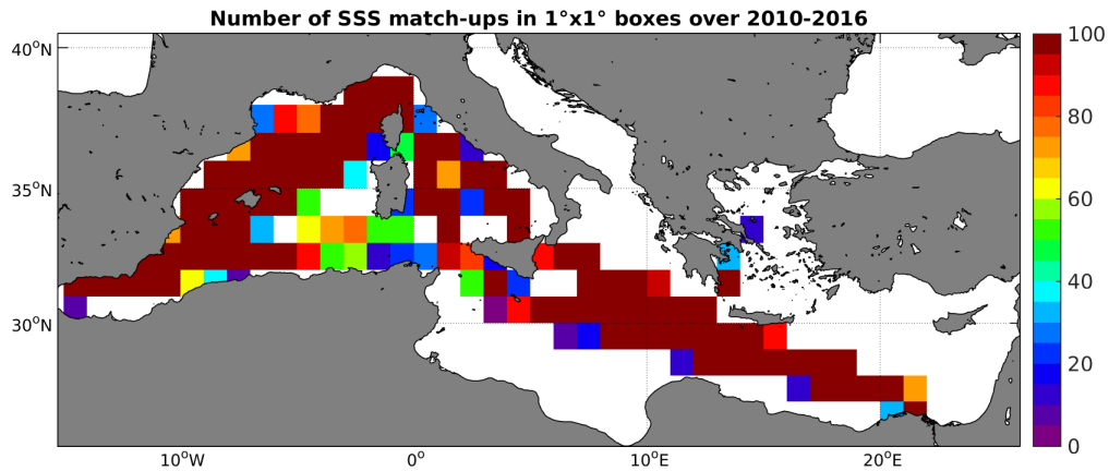
Figure 4: Number of SSS match-ups between TSG-LEGOS-DM SSS and the SMOS-L3-CATDS-CECOS-LOCEAN-V2-9DAYS-25KM SSS product for the Mediterranean Sea Pi-MEP region over 1°x1° boxes and for the full satellite product period.
