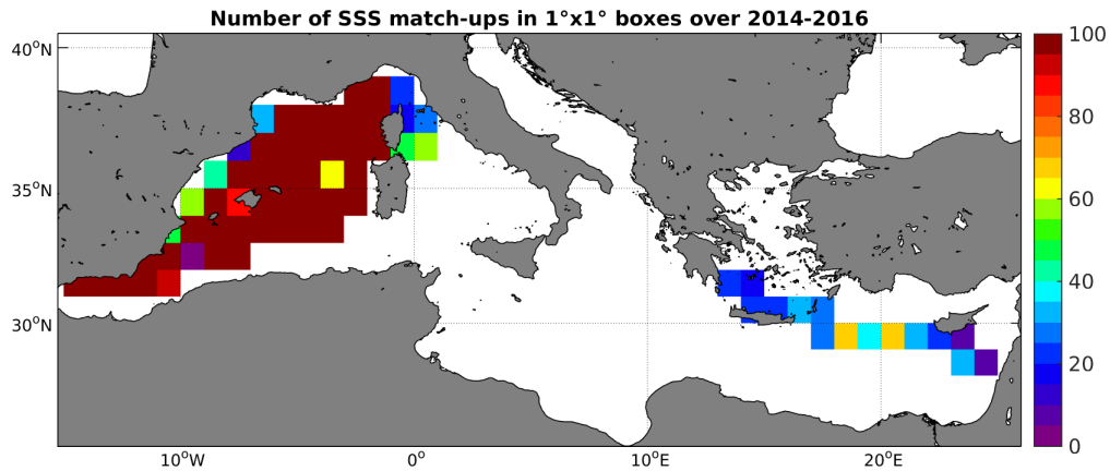
Figure 4: Number of SSS match-ups between TSG-GOSUD-Sailing-ship SSS and the SMOS-L3-CATDS-CECOS-LOCEAN-V2-9DAYS-25KM SSS product for the Mediterranean Sea Pi-MEP region over 1°x1° boxes and for the full satellite product period.
