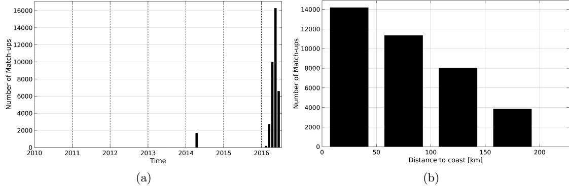
Figure 1: Number of match-ups between TSG-GOSUD-Sailing-ship and SMOS-L3-CATDS-CECOS-LOCEAN-V2-9DAYS-25KM SSS as a function of time (a) and as function of the distance to coast (b) over the Mediterranean Sea Pi-MEP region and for the full satellite product period.
