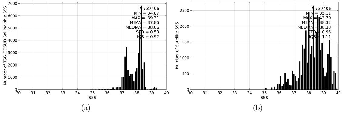
Figure 2: Histograms of SSS from TSG-GOSUD-Sailing-ship (a) and SMOS-L3-CATDS-CECOS-LOCEAN-V2-9DAYS-25KM (b) considering all match-up pairs per bins of 0.1 over the Mediterranean Sea Pi-MEP region and for the full satellite product period.
