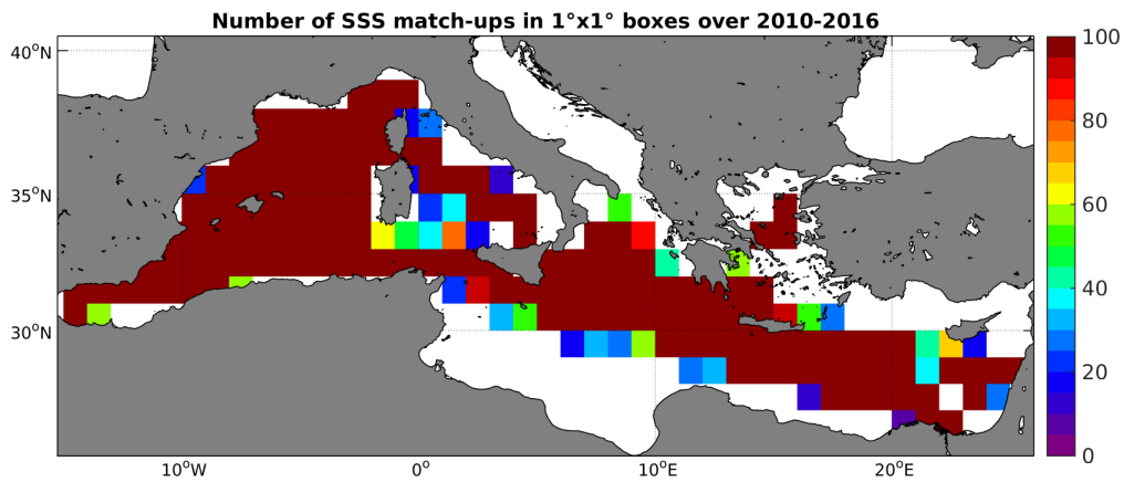
Figure 4: Number of SSS match-ups between TSG-GOSUD-Research-vessel SSS and the SMOS-L3-CATDS-CECOS-LOCEAN-V2-9DAYS-25KM SSS product for the Mediterranean Sea Pi-MEP region over 1^\circ \times 1^\circ boxes and for the full satellite product period.
