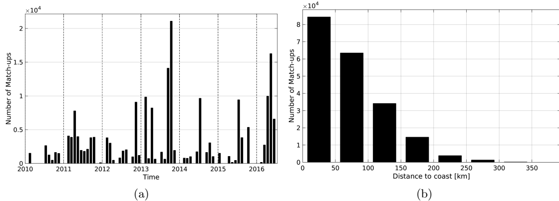
Figure 1: Number of match-ups between TSG-GOSUD-Research-vessel and SMOS-L3-CATDS-CECOS-LOCEAN-V2-9DAYS-25KM SSS as a function of time (a) and as function of the distance to coast (b) over the Mediterranean Sea Pi-MEP region and for the full satellite product period.
