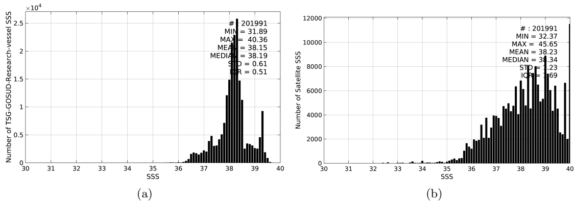
Figure 2: Histograms of SSS from TSG-GOSUD-Research-vessel (a) and SMOS-L3-CATDS-CECOS-LOCEAN-V2-9DAYS-25KM (b) considering all match-up pairs per bins of 0.1 over the Mediterranean Sea Pi-MEP region and for the full satellite product period.
