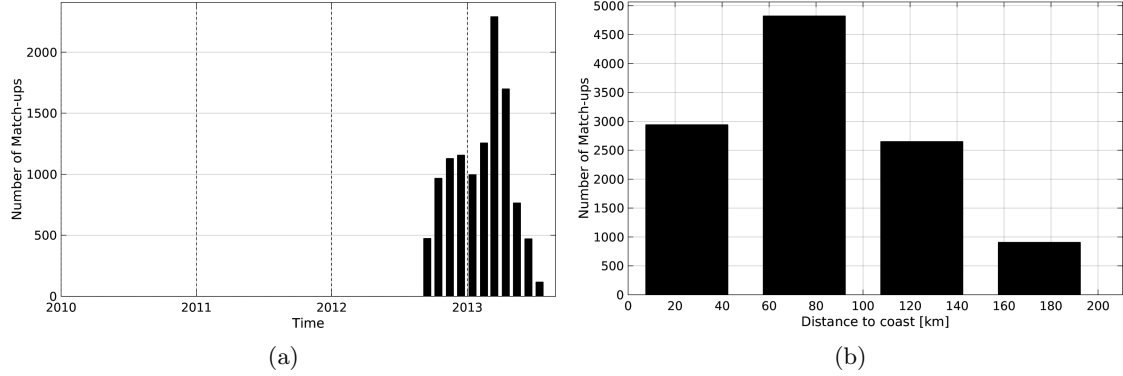
Figure 1: Number of match-ups between Surface drifters and SMOS-L3-CATDS-CECOS-LOCEAN-V2-9DAYS-25KM SSS as a function of time (a) and as function of the distance to coast (b) over the Mediterranean Sea Pi-MEP region and for the full satellite product period.
