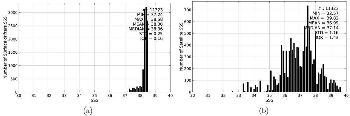
Figure 2: Histograms of SSS from Surface drifters (a) and SMOS-L3-CATDS-CECOS-LOCEAN-V2-9DAYS-25KM (b) considering all match-up pairs per bins of 0.1 over the Mediterranean Sea Pi-MEP region and for the full satellite product period.
