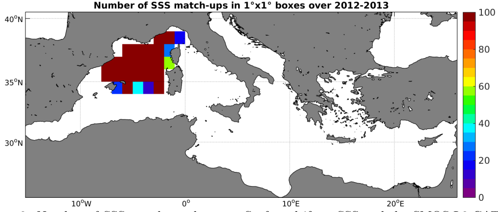
Figure 3: Number of SSS match-ups between Surface drifters SSS and the SMOS-L3-CATDS-CECOS-LOCEAN-V2-9DAYS-25KM SSS product for the Mediterranean Sea Pi-MEP region over 1°x1° boxes and for the full satellite product period.
