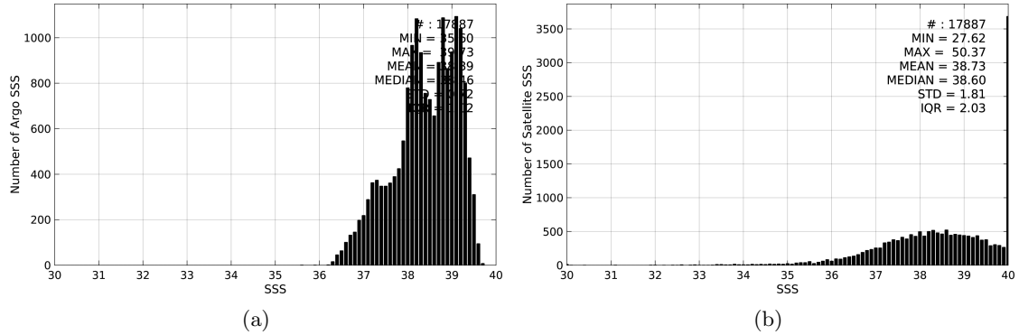
Figure 2: Histograms of SSS from Argo (a) and SMOS-L3-CATDS-CECOS-LOCEAN-V2-9DAYS-25KM (b) considering all match-up pairs per bins of 0.1 over the Mediterranean Sea Pi-MEP region and for the full satellite product period.
