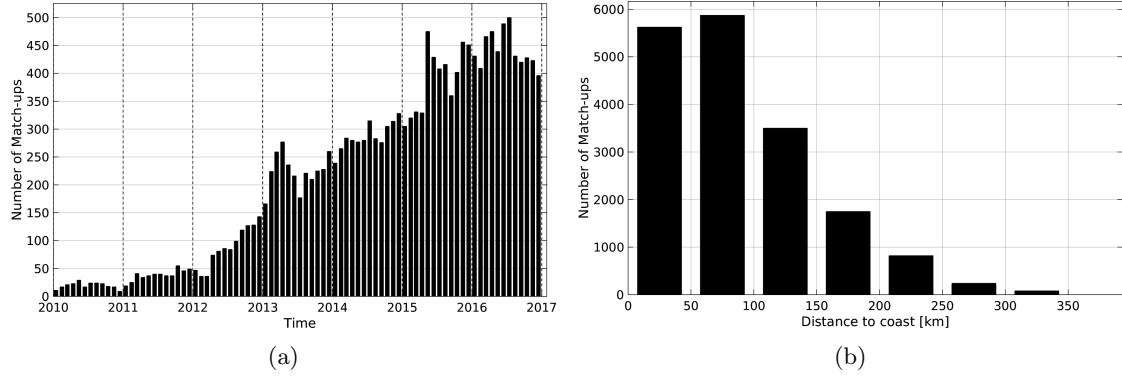
Figure 1: Number of match-ups between Argo and SMOS-L3-CATDS-CECOS-LOCEAN-V2-9DAYS-25KM SSS as a function of time (a) and as function of the distance to coast (b) over the Mediterranean Sea Pi-MEP region and for the full satellite product period.
