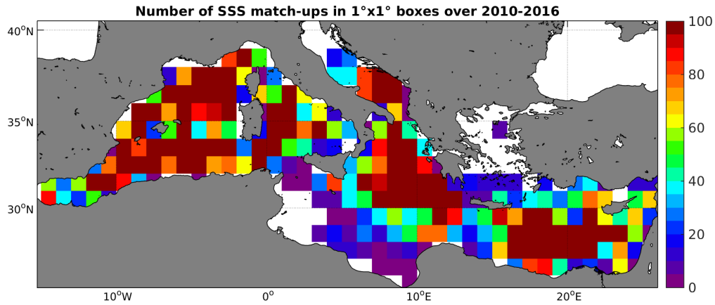
Figure 4: Number of SSS match-ups between Argo SSS and the SMOS-L3-CATDS-CECOS-LOCEAN-V2-9DAYS-25KM SSS product for the Mediterranean Sea Pi-MEP region over 1^\circ \times 1^\circ boxes and for the full satellite product period.
