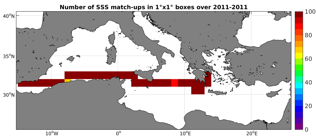
Figure 4: Number of SSS match-ups between TSG-SAMOS SSS and the SMOS-L3-CATDS-CECOS-LOCEAN-V2-18DAYS-25KM SSS product for the Mediterranean Sea Pi-MEP region over 1^\circ \times 1^\circ boxes and for the full satellite product period.
