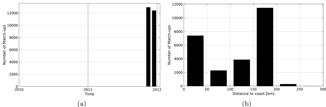
Figure 1: Number of match-ups between TSG-SAMOS and SMOS-L3-CATDS-CECOS-LOCEAN-V2-18DAYS-25KM SSS as a function of time (a) and as function of the distance to coast (b) over the Mediterranean Sea Pi-MEP region and for the full satellite product period.
