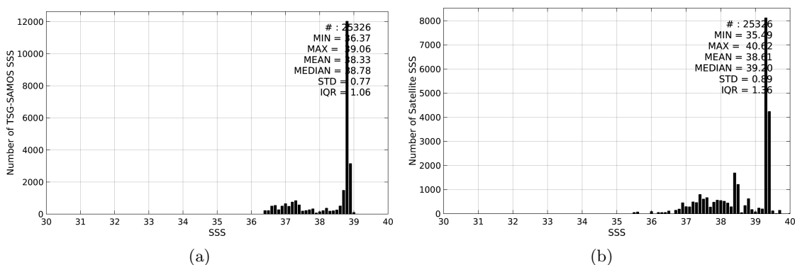
Figure 2: Histograms of SSS from TSG-SAMOS (a) and SMOS-L3-CATDS-CECOS-LOCEAN-V2-18DAYS-25KM (b) considering all match-up pairs per bins of 0.1 over the Mediterranean Sea Pi-MEP region and for the full satellite product period.
