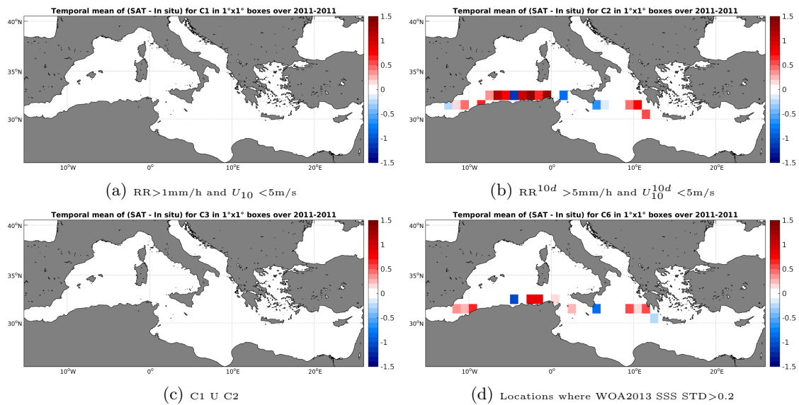
Figure 12: Temporal mean gridded over spatial boxes of size 1^\circ \times 1^\circ of \Delta SSS (SMOS-L3-CATDS-CECOS-LOCEAN-V2-18DAYS-25KM - TSG-SAMOS) for 4 different subdatasets corresponding to:RR > 1 mm/h and U_{10} < 5 m/s (a), RR ^{10d} > 5 mm/h and U_{10}^{10d} < 5 m/s (b), C1 U C2 (c),Locations where WOA2013 SSS STD > 0.2 (d).
