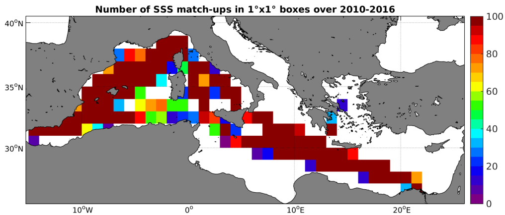
Figure 4: Number of SSS match-ups between TSG-LEGOS-DM SSS and the SMOS-L3-CATDS-CECOS-LOCEAN-V2-18DAYS-25KM SSS product for the Mediterranean Sea Pi-MEP region over 1^\circ \times 1^\circ boxes and for the full satellite product period.
