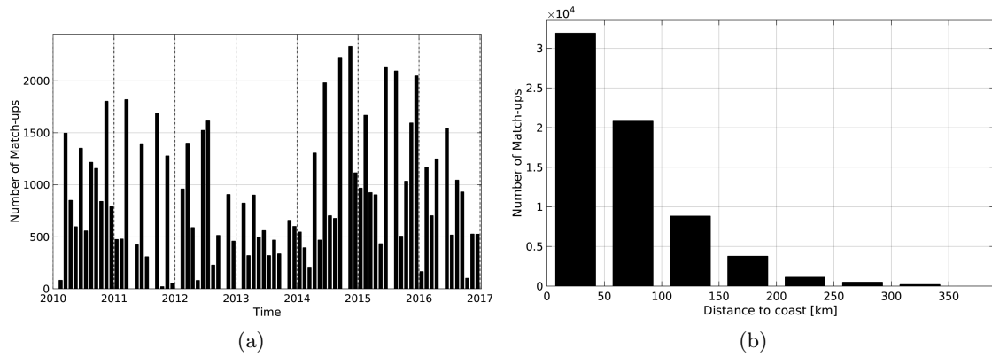
Figure 1: Number of match-ups between TSG-LEGOS-DM and SMOS-L3-CATDS-CECOS-LOCEAN-V2-18DAYS-25KM SSS as a function of time (a) and as function of the distance to coast (b) over the Mediterranean Sea Pi-MEP region and for the full satellite product period.
