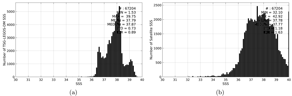
Figure 2: Histograms of SSS from TSG-LEGOS-DM (a) and SMOS-L3-CATDS-CECOS-LOCEAN-V2-18DAYS-25KM (b) considering all match-up pairs per bins of 0.1 over the Mediterranean Sea Pi-MEP region and for the full satellite product period.
