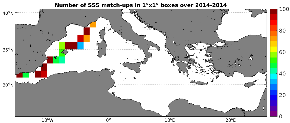
Figure 4: Number of SSS match-ups between TSG-GOSUD-Sailing-ship SSS and the SMOS-L3-CATDS-CECOS-LOCEAN-V2-18DAYS-25KM SSS product for the Mediterranean Sea Pi-MEP region over 1^\circ \times 1^\circ boxes and for the full satellite product period.
