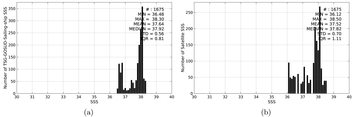
Figure 2: Histograms of SSS from TSG-GOSUD-Sailing-ship (a) and SMOS-L3-CATDS-CECOS-LOCEAN-V2-18DAYS-25KM (b) considering all match-up pairs per bins of 0.1 over the Mediterranean Sea Pi-MEP region and for the full satellite product period.
