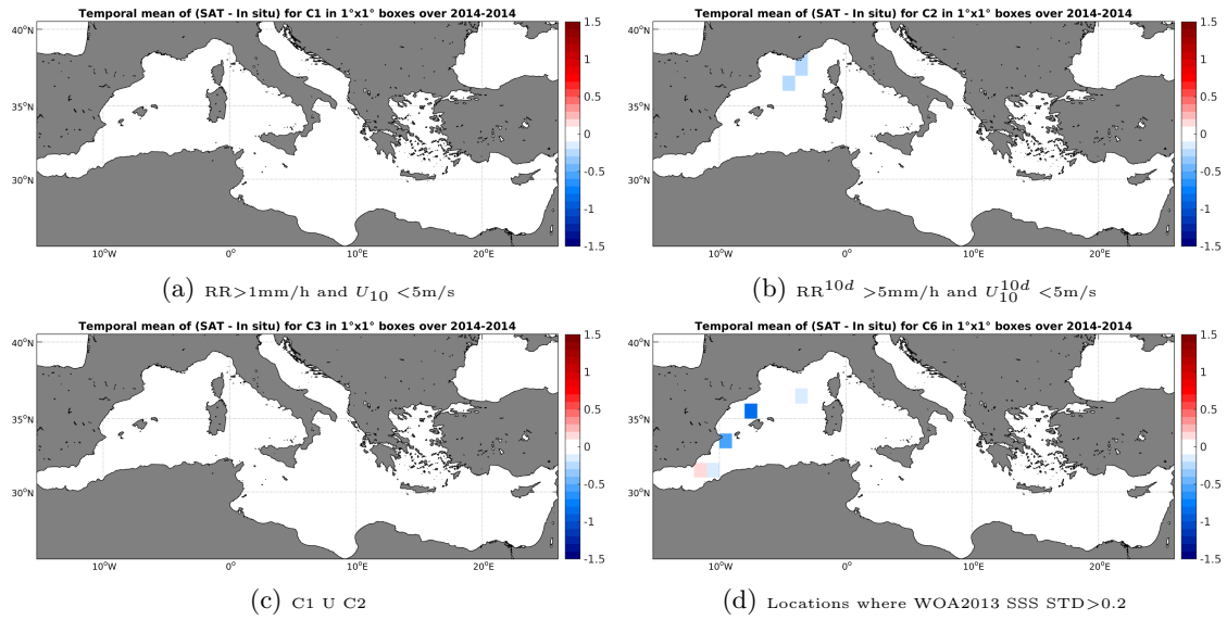
Figure 12: Temporal mean gridded over spatial boxes of size 1^\circ \times 1^\circ of \Delta SSS (SMOS-L3-CATDS-CECOS-LOCEAN-V2-18DAYS-25KM - TSG-GOSUD-Sailing-ship) for 4 different subdatasets corresponding to: RR > 1\text{mm/h} and U_{10} < 5\text{m/s} (a), RR^{10d} > 5\text{mm/h} and U_{10}^{10d} < 5\text{m/s} (b), C1 U C2 (c), Locations where WOA2013 SSS STD > 0.2 (d).
