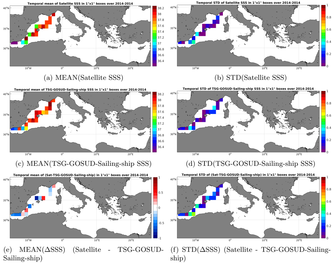
Figure 6: Temporal mean (left) and STD (right) of SSS from SMOS-L3-CATDS-CECOS-LOCEAN-V2-18DAYS-25KM (top), TSG-GOSUD-Sailing-ship (middle), and of \Delta SSS (Satellite - TSG-GOSUD-Sailing-ship). Only match-up pairs are used to generate these maps.
