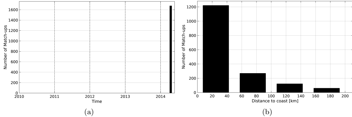
Figure 1: Number of match-ups between TSG-GOSUD-Sailing-ship and SMOS-L3-CATDS-CECOS-LOCEAN-V2-18DAYS-25KM SSS as a function of time (a) and as function of the distance to coast (b) over the Mediterranean Sea Pi-MEP region and for the full satellite product period.
