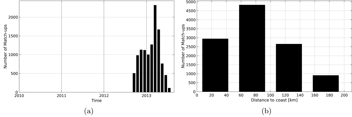
Figure 1: Number of match-ups between Surface drifters and SMOS-L3-CATDS-CECOS-LOCEAN-V2-18DAYS-25KM SSS as a function of time (a) and as function of the distance to coast (b) over the Mediterranean Sea Pi-MEP region and for the full satellite product period.
