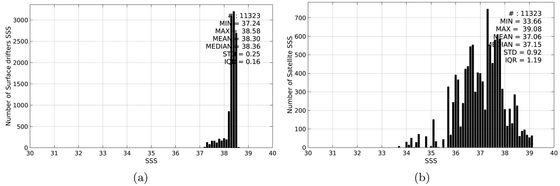
Figure 2: Histograms of SSS from Surface drifters (a) and SMOS-L3-CATDS-CECOS-LOCEAN-V2-18DAYS-25KM (b) considering all match-up pairs per bins of 0.1 over the Mediterranean Sea Pi-MEP region and for the full satellite product period.
