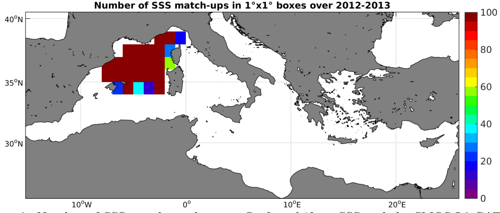
Figure 3: Number of SSS match-ups between Surface drifters SSS and the SMOS-L3-CATDS-CECOS-LOCEAN-V2-18DAYS-25KM SSS product for the Mediterranean Sea Pi-MEP region over 1°x1° boxes and for the full satellite product period.
