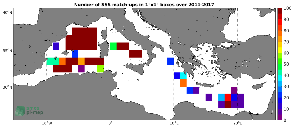
Figure 4: Number of SSS match-ups between TSG (GOSUD-Research-vessel) SSS and the SMOS SSS L3 v2 - Monthly - 0.25 Deg (CATDS-CECOS-IFREMER) SSS product for the Mediterranean Sea Pi-MEP region over 1^\circ \times 1^\circ boxes and for the full satellite product period.
