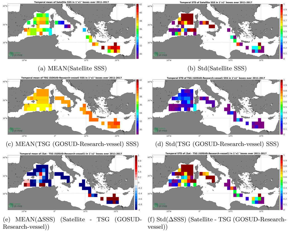
Figure 6: Temporal mean (left) and Std (right) of SSS from SMOS SSS L3 v2 - Monthly - 0.25 Deg (CATDS-CECOS-IFREMER) (top), TSG (GOSUD-Research-vessel) (middle), and of \Delta SSS (Satellite - TSG (GOSUD-Research-vessel)). Only match-up pairs are used to generate these maps.
