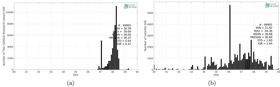
Figure 2: Histograms of SSS from TSG (GOSUD-Research-vessel) (a) and SMOS SSS L3 v2 - Monthly - 0.25 Deg (CATDS-CECOS-IFREMER) (b) considering all match-up pairs per bins of 0.1 over the Mediterranean Sea Pi-MEP region and for the full satellite product period.
