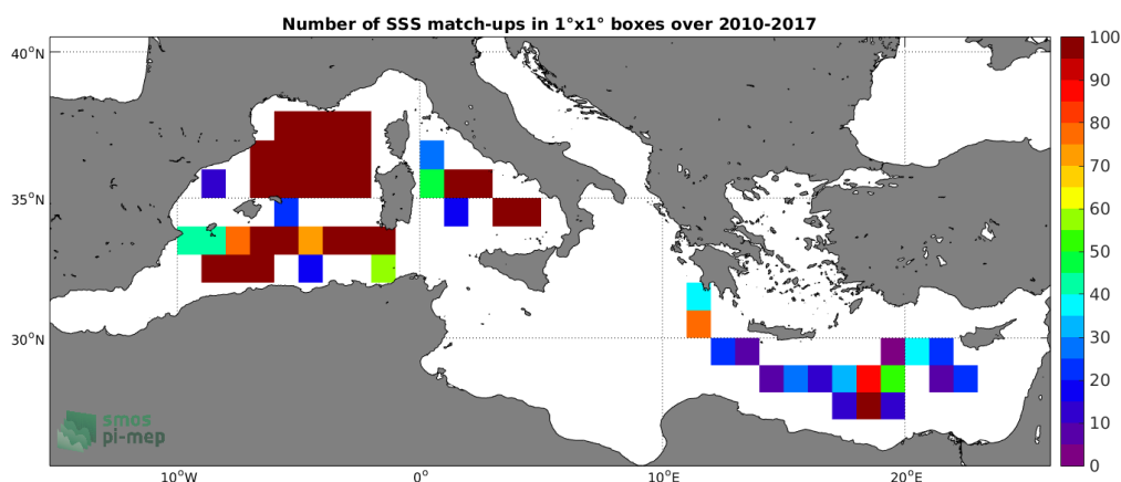
Figure 4: Number of SSS match-ups between TSG-GOSUD-Research-vessel SSS and the SMOS L3 v2 - Monthly - 0.25 Deg (CATDS-CECOS-IFREMER) SSS product for the Mediterranean Sea Pi-MEP region over 1^\circ \times 1^\circ boxes and for the full satellite product period.
