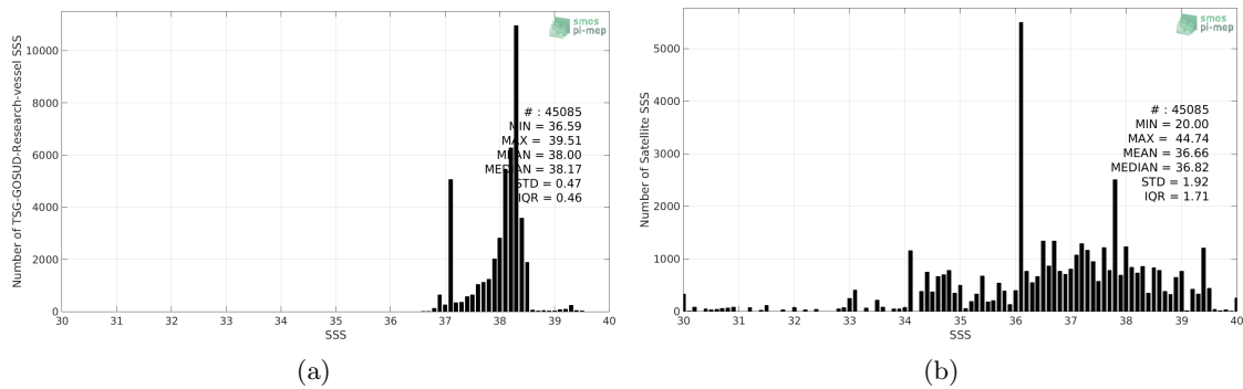
Figure 2: Histograms of SSS from TSG-GOSUD-Research-vessel (a) and SMOS L3 v2 - Monthly - 0.25 Deg (CATDS-CECOS-IFREMER) (b) considering all match-up pairs per bins of 0.1 over the Mediterranean Sea Pi-MEP region and for the full satellite product period.
