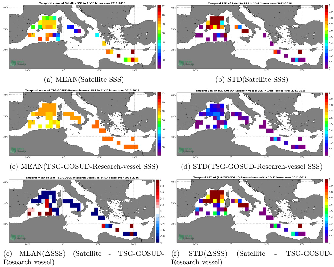
Figure 6: Temporal mean (left) and STD (right) of SSS from SMOS-L3-CATDS-IFREMER-CECOS-V2-MONTHLY-0.25DEG (top), TSG-GOSUD-Research-vessel (middle), and of \Delta SSS (Satellite - TSG-GOSUD-Research-vessel). Only match-up pairs are used to generate these maps.
