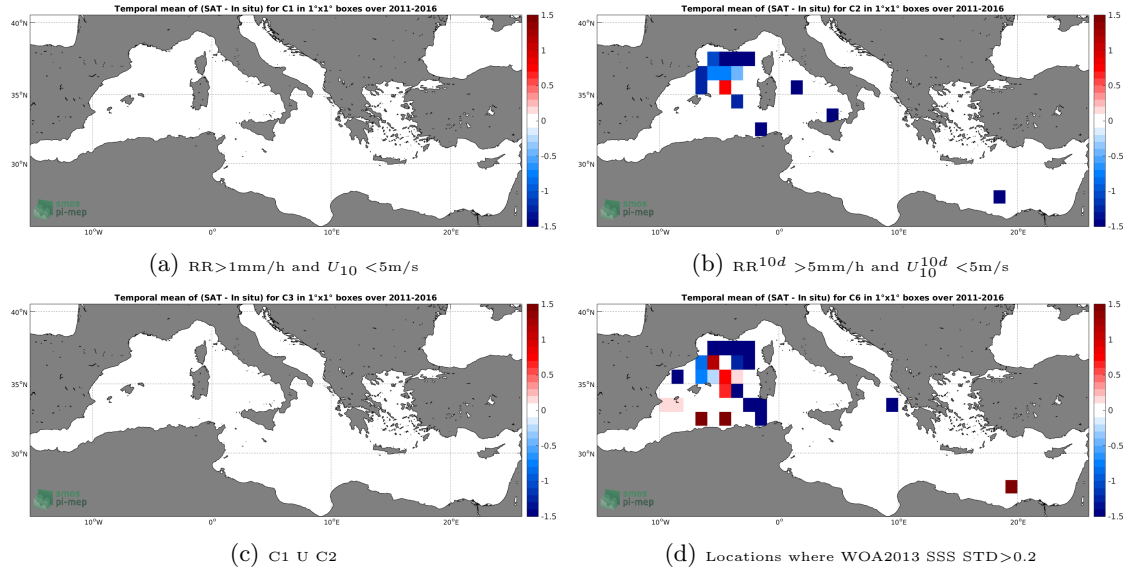
Figure 12: Temporal mean gridded over spatial boxes of size 1^\circ \times 1^\circ of \Delta SSS (SMOS-L3-CATDS-IFREMER-CECOS-V2-MONTHLY-0.25DEG - TSG-GOSUD-Research-vessel) for 4 different subdatasets corresponding to: RR > 1\text{mm/h} and U_{10} < 5\text{m/s} (a), RR^{10d} > 5\text{mm/h} and U_{10}^{10d} < 5\text{m/s} (b), C1 U C2 (c), Locations where WOA2013 SSS STD > 0.2 (d).
