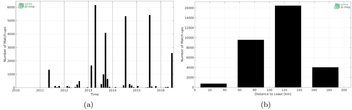
Figure 1: Number of match-ups between TSG-GOSUD-Research-vessel and SMOS-L3-CATDS-IFREMER-CECOS-V2-MONTHLY-0.25DEG SSS as a function of time (a) and as function of the distance to coast (b) over the Mediterranean Sea Pi-MEP region and for the full satellite product period.
