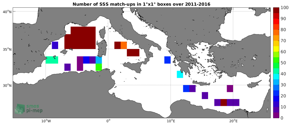
Figure 4: Number of SSS match-ups between TSG-GOSUD-Research-vessel SSS and the SMOS-L3-CATDS-IFREMER-CECOS-V2-MONTHLY-0.25DEG SSS product for the Mediterranean Sea Pi-MEP region over 1^\circ \times 1^\circ boxes and for the full satellite product period.
