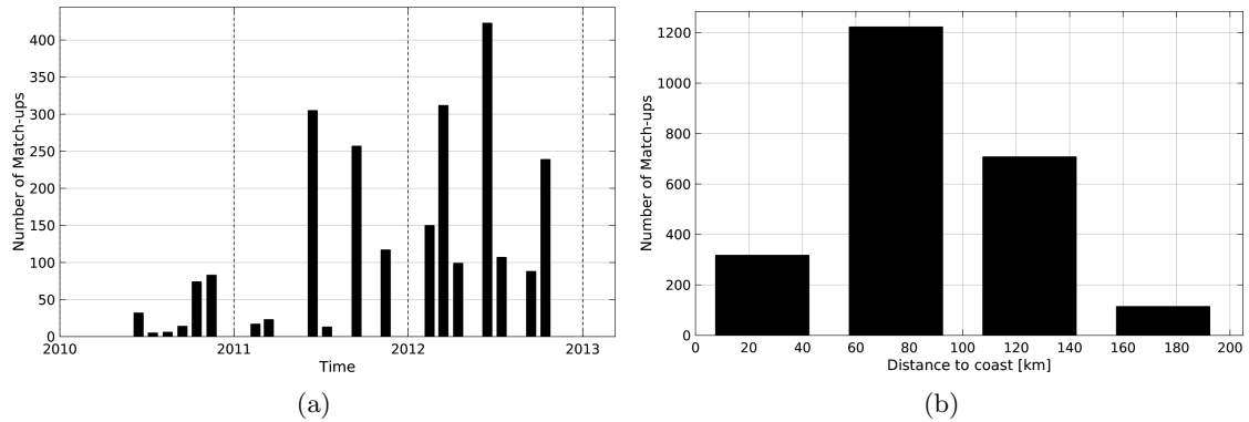
Figure 1: Number of match-ups between TSG-LEGOS-DM and SMOS-L3-CATDS-CECOS-IFREMER-V2-1DAY-0.5deg SSS as a function of time (a) and as function of the distance to coast (b) over the Mediterranean Sea Pi-MEP region and for the full satellite product period.
