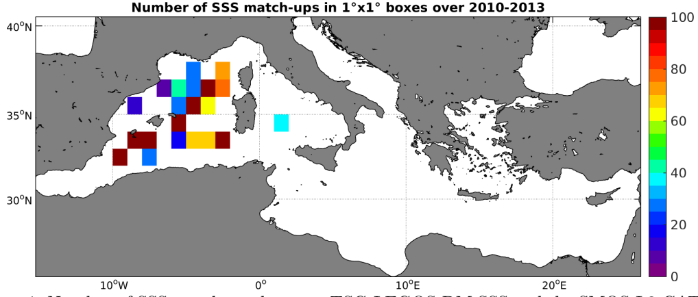
Figure 4: Number of SSS match-ups between TSG-LEGOS-DM SSS and the SMOS-L3-CATDS-CECOS-IFREMER-V2-1DAY-0.5deg SSS product for the Mediterranean Sea Pi-MEP region over 1°x1° boxes and for the full satellite product period.
