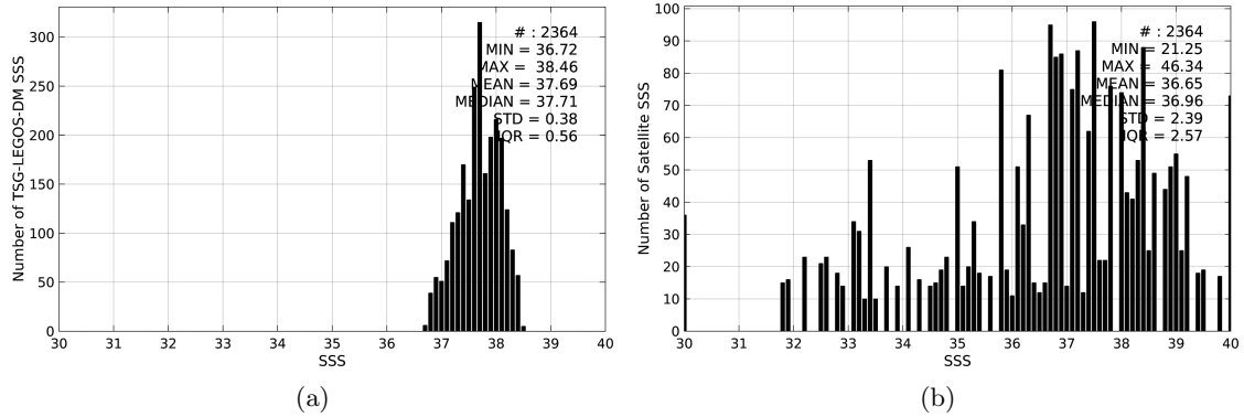
Figure 2: Histograms of SSS from TSG-LEGOS-DM (a) and SMOS-L3-CATDS-CECOS-IFREMER-V2-1DAY-0.5deg (b) considering all match-up pairs per bins of 0.1 over the Mediterranean Sea Pi-MEP region and for the full satellite product period.
