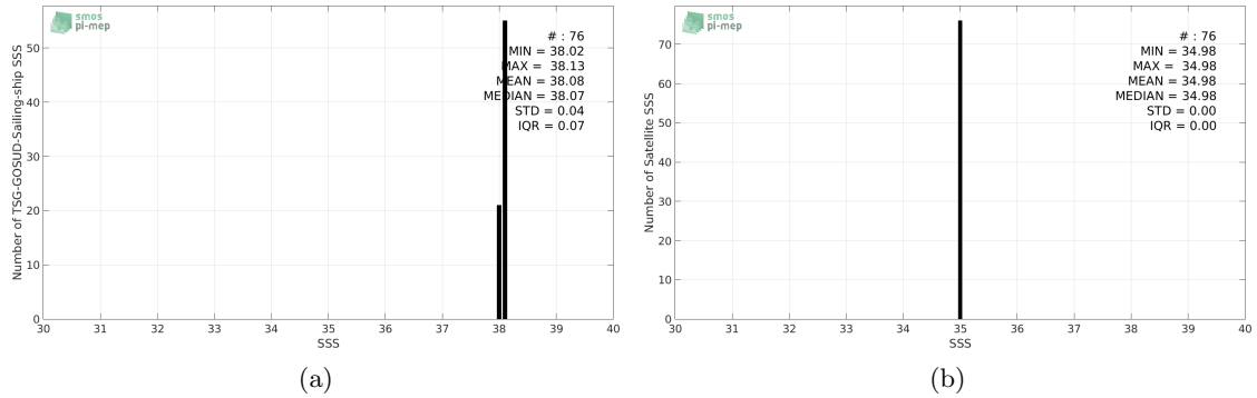
Figure 2: Histograms of SSS from TSG-GOSUD-Sailing-ship (a) and SMOS-L3-CATDS-CECOS-IFREMER-V2-1DAY-0.5DEG (b) considering all match-up pairs per bins of 0.1 over the Mediterranean Sea Pi-MEP region and for the full satellite product period.
