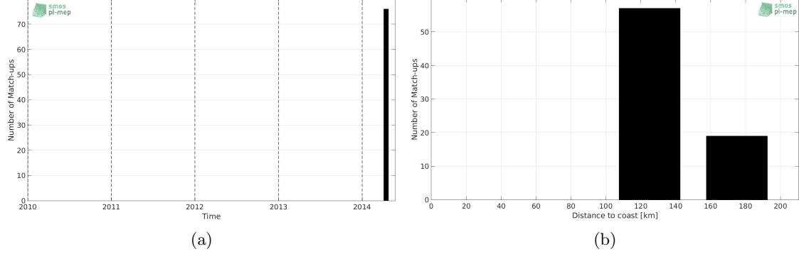
Figure 1: Number of match-ups between TSG-GOSUD-Sailing-ship and SMOS-L3-CATDS-CECOS-IFREMER-V2-1DAY-0.5DEG SSS as a function of time (a) and as function of the distance to coast (b) over the Mediterranean Sea Pi-MEP region and for the full satellite product period.
