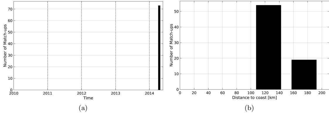
Figure 1: Number of match-ups between TSG-GOSUD-Sailing-ship and SMOS-L3-CATDS-CECOS-IFREMER-V2-1DAY-0.5DEG SSS as a function of time (a) and as function of the distance to coast (b) over the Mediterranean Sea Pi-MEP region and for the full satellite product period.
