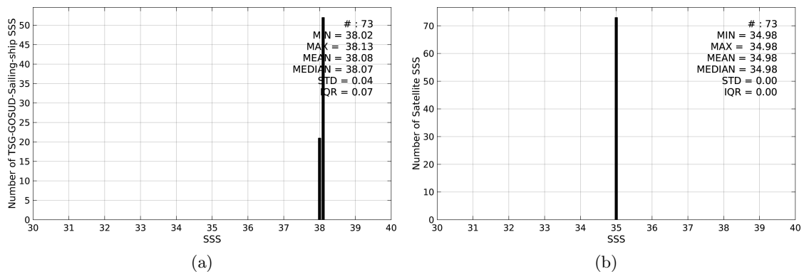
Figure 2: Histograms of SSS from TSG-GOSUD-Sailing-ship (a) and SMOS-L3-CATDS-CECOS-IFREMER-V2-1DAY-0.5DEG (b) considering all match-up pairs per bins of 0.1 over the Mediterranean Sea Pi-MEP region and for the full satellite product period.
