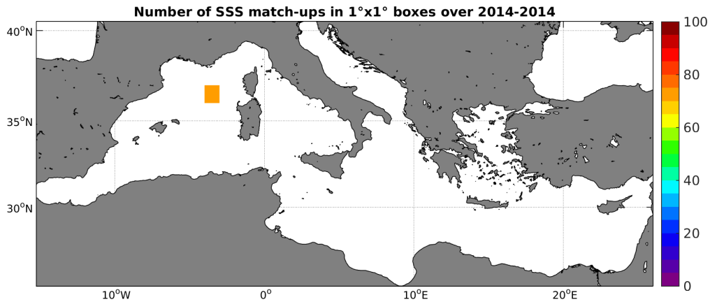
Figure 4: Number of SSS match-ups between TSG-GOSUD-Sailing-ship SSS and the SMOS-L3-CATDS-CECOS-IFREMER-V2-1DAY-0.5DEG SSS product for the Mediterranean Sea Pi-MEP region over 1^\circ \times 1^\circ boxes and for the full satellite product period.
