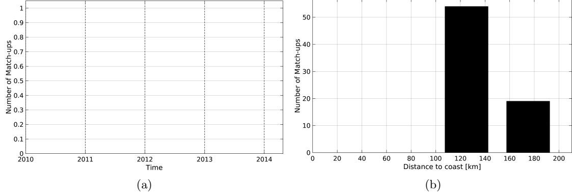
Figure 1: Number of match-ups between TSG-GOSUD-Sailing-ship and SMOS-L3-CATDS-CECOS-IFREMER-V2-1DAY-0.5deg SSS as a function of time (a) and as function of the distance to coast (b) over the Mediterranean Sea Pi-MEP region and for the full satellite product period.
