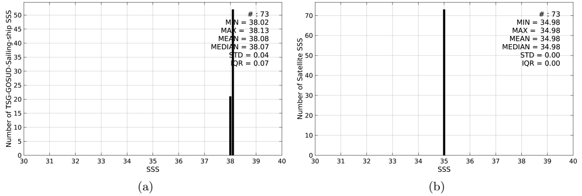
Figure 2: Histograms of SSS from TSG-GOSUD-Sailing-ship (a) and SMOS-L3-CATDS-CECOS-IFREMER-V2-1DAY-0.5deg (b) considering all match-up pairs per bins of 0.1 over the Mediterranean Sea Pi-MEP region and for the full satellite product period.
