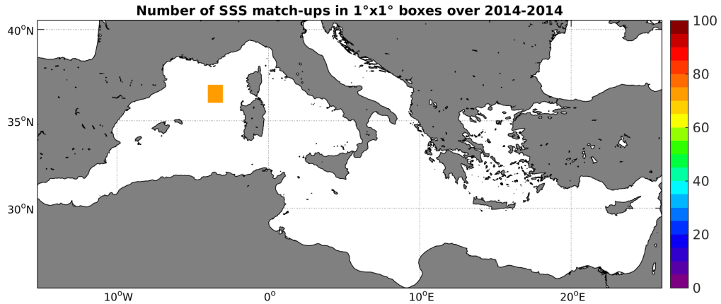
Figure 4: Number of SSS match-ups between TSG-GOSUD-Sailing-ship SSS and the SMOS-L3-CATDS-CECOS-IFREMER-V2-1DAY-0.5deg SSS product for the Mediterranean Sea Pi-MEP region over 1°x1° boxes and for the full satellite product period.
