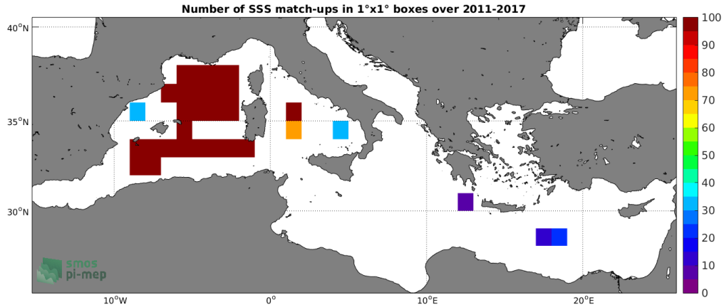
Figure 4: Number of SSS match-ups between TSG-GOSUD-Research-vessel SSS and the SMOS L3 v2 - Daily - 0.5 Deg (CATDS-CECOS-IFREMER) SSS product for the Mediterranean Sea Pi-MEP region over 1°x1° boxes and for the full satellite product period.
