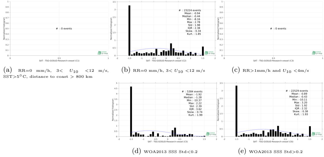
Figure 13: Normalized histogram of \Delta SSS (SMOS L3 v2 - Daily - 0.5 Deg (CATDS-CECOS-IFREMER) - TSG-GOSUD-Research-vessel) for 5 different subdatasets corresponding to: RR=0 mm/h, 3 < U_{10} < 12 m/s, SST>5°C, distance to coast > 800 km (a), RR=0 mm/h, 3 < U_{10} < 12 m/s (b), RR>1mm/h and U_{10} < 4 m/s (c), WOA2013 SSS Std<0.2 (d), WOA2013 SSS Std>0.2 (e).
