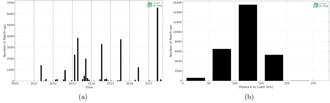
Figure 1: Number of match-ups between TSG-GOSUD-Research-vessel and SMOS L3 v2 - Daily - 0.5 Deg (CATDS-CECOS-IFREMER) SSS as a function of time (a) and as function of the distance to coast (b) over the Mediterranean Sea Pi-MEP region and for the full satellite product period.
