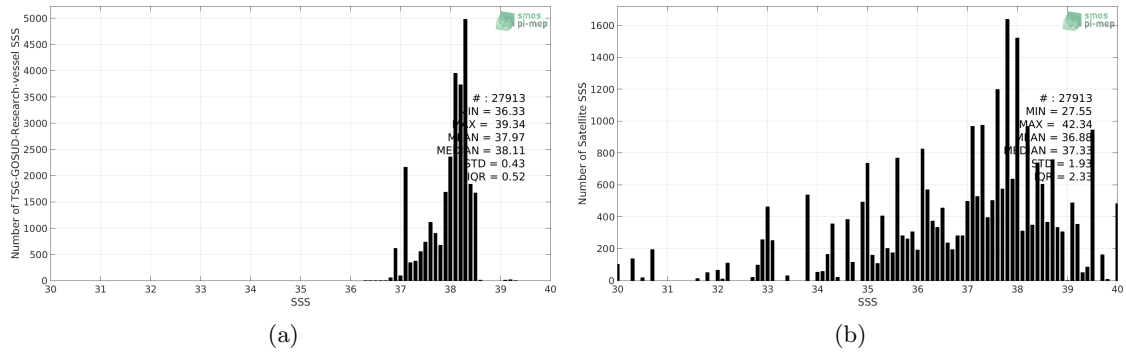
Figure 2: Histograms of SSS from TSG-GOSUD-Research-vessel (a) and SMOS L3 v2 - Daily - 0.5 Deg (CATDS-CECOS-IFREMER) (b) considering all match-up pairs per bins of 0.1 over the Mediterranean Sea Pi-MEP region and for the full satellite product period.
