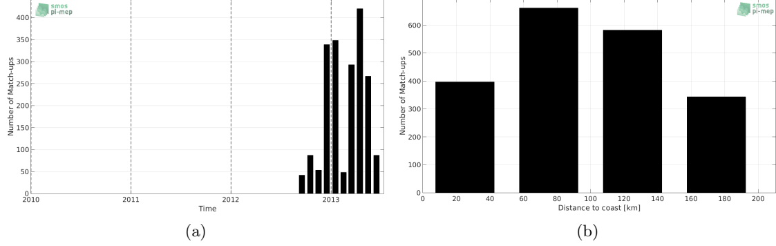
Figure 1: Number of match-ups between Surface drifters and SMOS-L3-CATDS-CECOS-IFREMER-V2-1DAY-0.5DEG SSS as a function of time (a) and as function of the distance to coast (b) over the Mediterranean Sea Pi-MEP region and for the full satellite product period.
