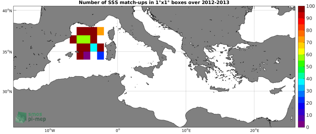
Figure 3: Number of SSS match-ups between Surface drifters SSS and the SMOS-L3-CATDS-CECOS-IFREMER-V2-1DAY-0.5DEG SSS product for the Mediterranean Sea Pi-MEP region over 1°x1° boxes and for the full satellite product period.
