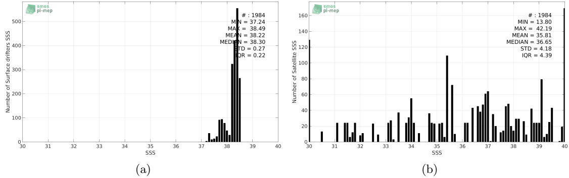
Figure 2: Histograms of SSS from Surface drifters (a) and SMOS-L3-CATDS-CECOS-IFREMER-V2-1DAY-0.5DEG (b) considering all match-up pairs per bins of 0.1 over the Mediterranean Sea Pi-MEP region and for the full satellite product period.
