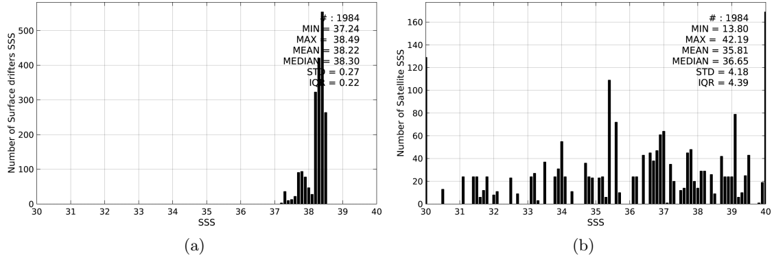
Figure 2: Histograms of SSS from Surface drifters (a) and SMOS-L3-CATDS-CECOS-IFREMER-V2-1DAY-0.5deg (b) considering all match-up pairs per bins of 0.1 over the Mediterranean Sea Pi-MEP region and for the full satellite product period.
