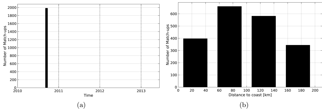
Figure 1: Number of match-ups between Surface drifters and SMOS-L3-CATDS-CECOS-IFREMER-V2-1DAY-0.5deg SSS as a function of time (a) and as function of the distance to coast (b) over the Mediterranean Sea Pi-MEP region and for the full satellite product period.
