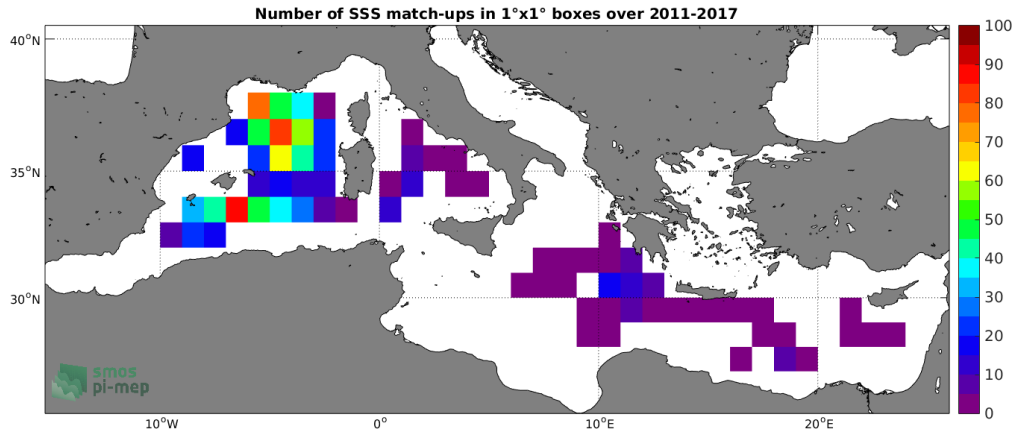
Figure 4: Number of SSS match-ups between Argo SSS and the SMOS L3 v2 - Daily - 0.5 Deg (CATDS-CECOS-IFREMER) SSS product for the Mediterranean Sea Pi-MEP region over 1^\circ \times 1^\circ boxes and for the full satellite product period.
