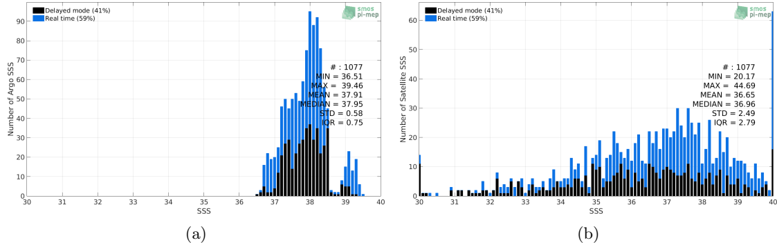
Figure 2: Histograms of SSS from Argo (a) and SMOS L3 v2 - Daily - 0.5 Deg (CATDS-CECOS-IFREMER) (b) considering all match-up pairs per bins of 0.1 over the Mediterranean Sea Pi-MEP region and for the full satellite product period.
