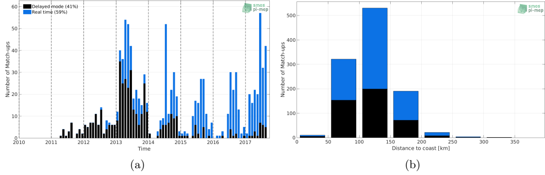
Figure 1: Number of match-ups between Argo and SMOS L3 v2 - Daily - 0.5 Deg (CATDS-CECOS-IFREMER) SSS as a function of time (a) and as function of the distance to coast (b) over the Mediterranean Sea Pi-MEP region and for the full satellite product period.
