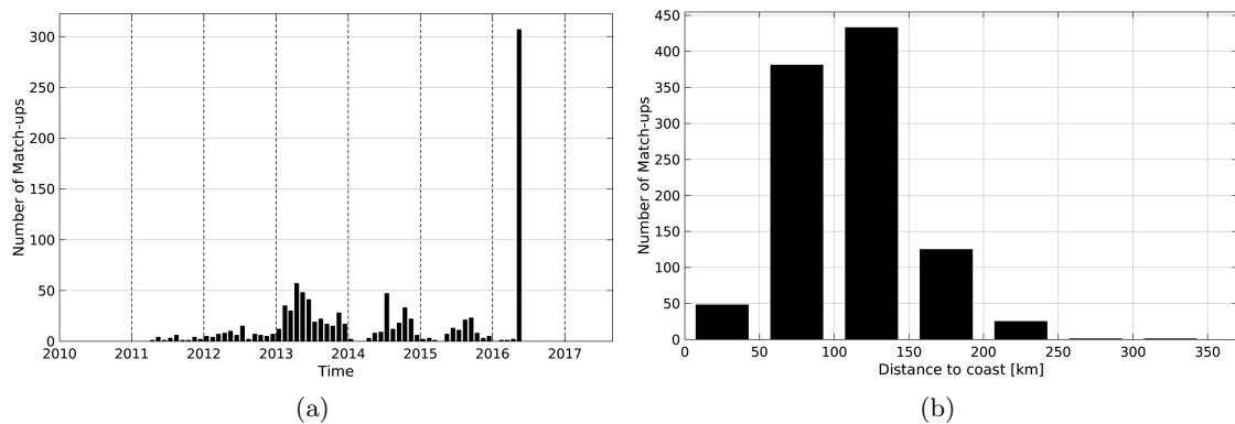
Figure 1: Number of match-ups between Argo and SMOS-L3-CATDS-CECOS-IFREMER-V2-1DAY-0.5deg SSS as a function of time (a) and as function of the distance to coast (b) over the Mediterranean Sea Pi-MEP region and for the full satellite product period.
