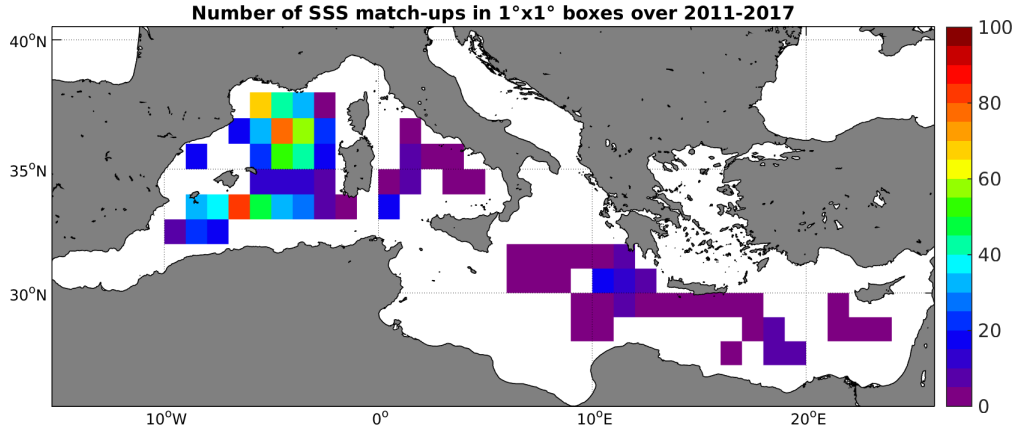
Figure 4: Number of SSS match-ups between Argo SSS and the SMOS-L3-CATDS-CECOS-IFREMER-V2-1DAY-0.5deg SSS product for the Mediterranean Sea Pi-MEP region over 1^\circ \times 1^\circ boxes and for the full satellite product period.
