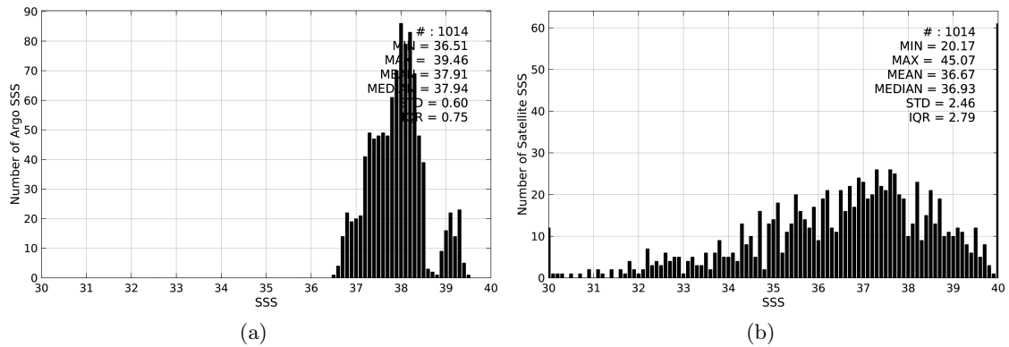
Figure 2: Histograms of SSS from Argo (a) and SMOS-L3-CATDS-CECOS-IFREMER-V2-1DAY-0.5deg (b) considering all match-up pairs per bins of 0.1 over the Mediterranean Sea Pi-MEP region and for the full satellite product period.
