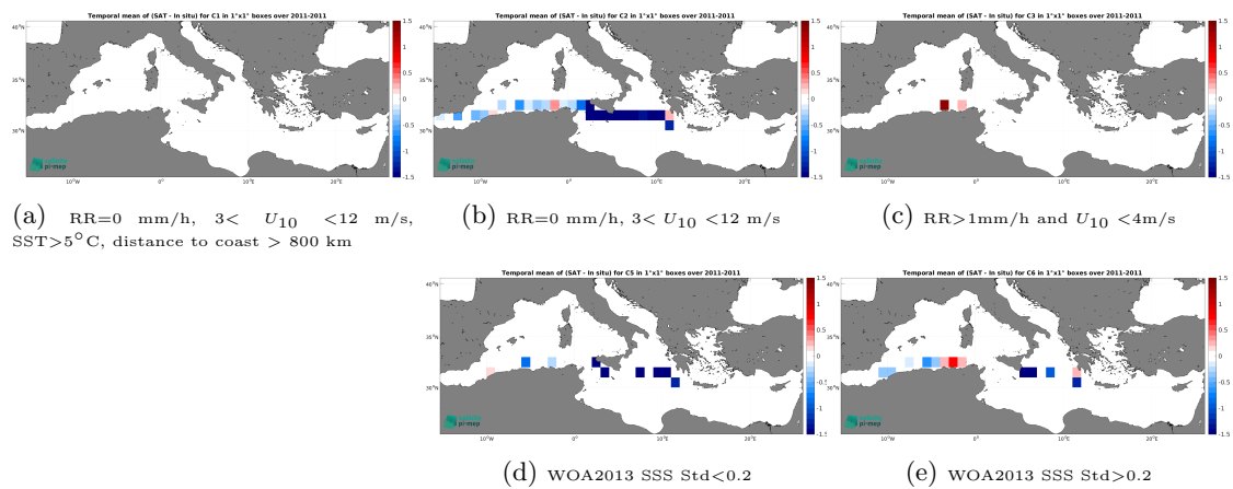
Figure 14: Temporal mean gridded over spatial boxes of size 1^\circ \times 1^\circ of \Delta\text{SSS} (SMOS SSS L3 v335 - Monthly - 25 km (CATDS-CPDC) - TSG (SAMOS)) for 5 different subdatasets corresponding to:RR=0 mm/h, 3 < U_{10} < 12 m/s, SST>5°C, distance to coast > 800 km (a), RR=0 mm/h, 3 < U_{10} < 12 m/s (b), RR>1mm/h and U_{10} < 4 m/s (c), WOA2013 SSS Std<0.2 (d), WOA2013 SSS Std>0.2 (e).
