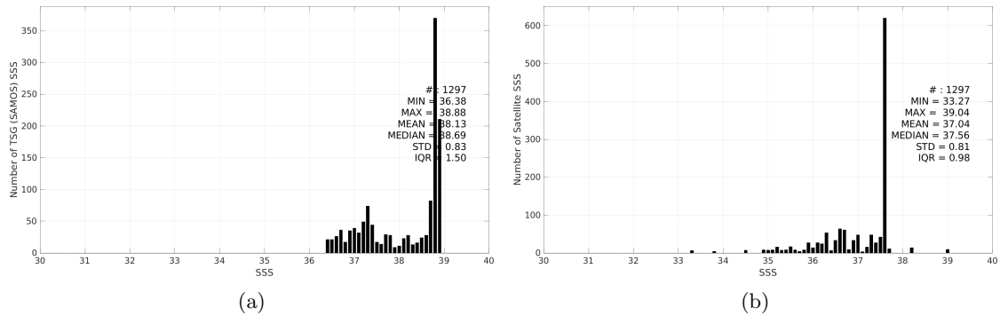
Figure 3: Histograms of SSS from TSG (SAMOS) (a) and SMOS SSS L3 v335 - Monthly - 25 km (CATDS-CPDC) (b) considering all match-up pairs per bins of 0.1 over the Mediterranean Sea Pi-MEP region and for the full satellite product period.
