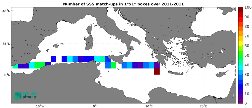
Figure 5: Number of SSS match-ups between TSG (SAMOS) SSS and the SMOS SSS L3 v335 - Monthly - 25 km (CATDS-CPDC) SSS product for the Mediterranean Sea Pi-MEP region over 1^\circ \times 1^\circ boxes and for the full satellite product period.
