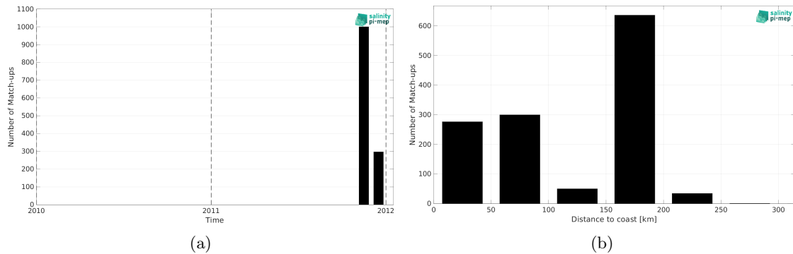
Figure 2: Number of match-ups between TSG (SAMOS) and SMOS SSS L3 v335 - Monthly - 25 km (CATDS-CPDC) SSS as a function of time (a) and as function of the distance to coast (b) over the Mediterranean Sea Pi-MEP region and for the full satellite product period.
