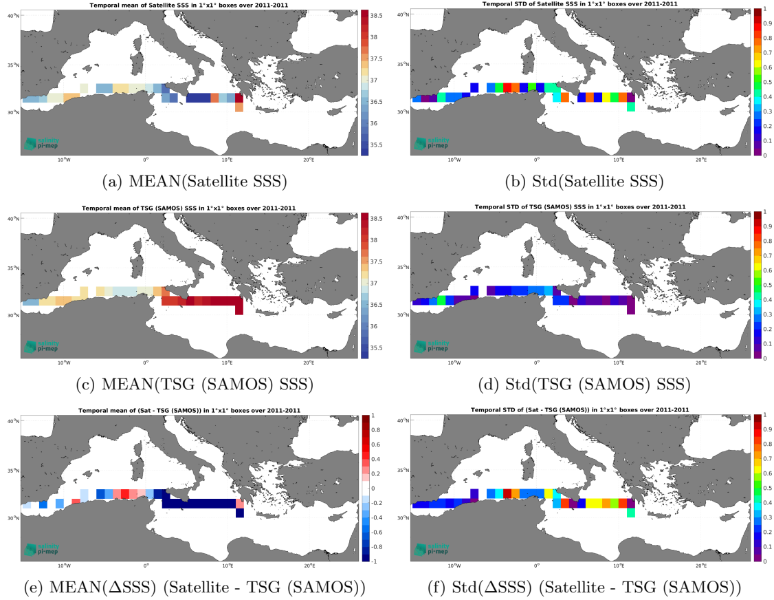
Figure 6: Temporal mean (left) and Std (right) of SSS from SMOS SSS L3 v335 - Monthly - 25 km (CATDS-CPDC) (top), TSG (SAMOS) (middle), and of \Delta\text{SSS} (Satellite - TSG (SAMOS)). Only match-up pairs are used to generate these maps.
