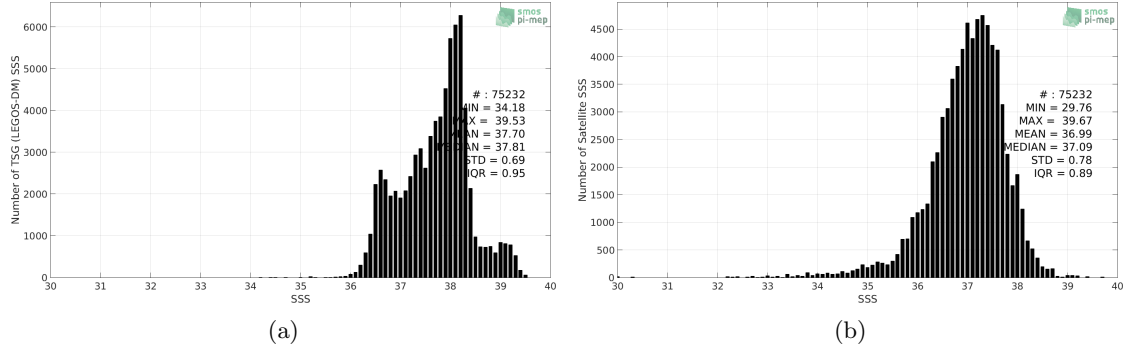
Figure 2: Histograms of SSS from TSG (LEGOS-DM) (a) and SMOS SSS L3 v335 - Monthly - 25 km (CATDS-CPDC) (b) considering all match-up pairs per bins of 0.1 over the Mediterranean Sea Pi-MEP region and for the full satellite product period.
