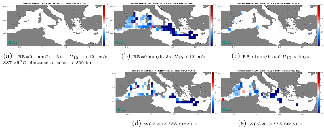
Figure 14: Temporal mean gridded over spatial boxes of size 1^\circ \times 1^\circ of \Delta\text{SSS} (SMOS SSS L3 v335 - Monthly - 25 km (CATDS-CPDC) - TSG (CSIC-UTM)) for 5 different subdatasets corresponding to:RR=0 mm/h, 3 < U_{10} < 12 m/s, SST>5°C, distance to coast > 800 km (a), RR=0 mm/h, 3 < U_{10} < 12 m/s (b), RR>1mm/h and U_{10} < 4 m/s (c), WOA2013 SSS Std<0.2 (d), WOA2013 SSS Std>0.2 (e).
